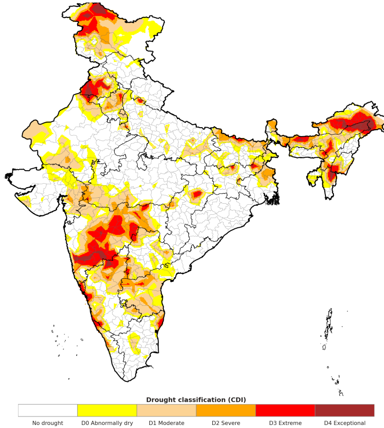
Combined Drought Index (CDI) for the week ending September 30, 2026.
