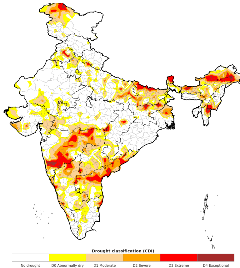
Combined Drought Index (CDI) for the week ending September 2, 2026.
