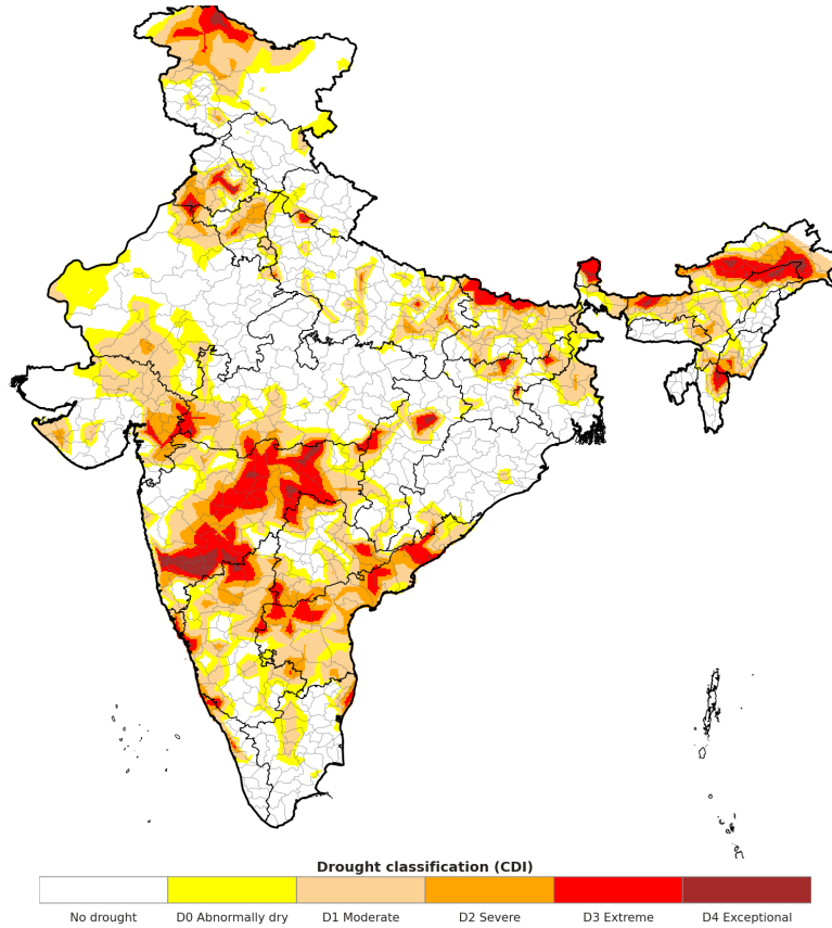
Combined Drought Index (CDI) for the week ending September 16, 2026.
