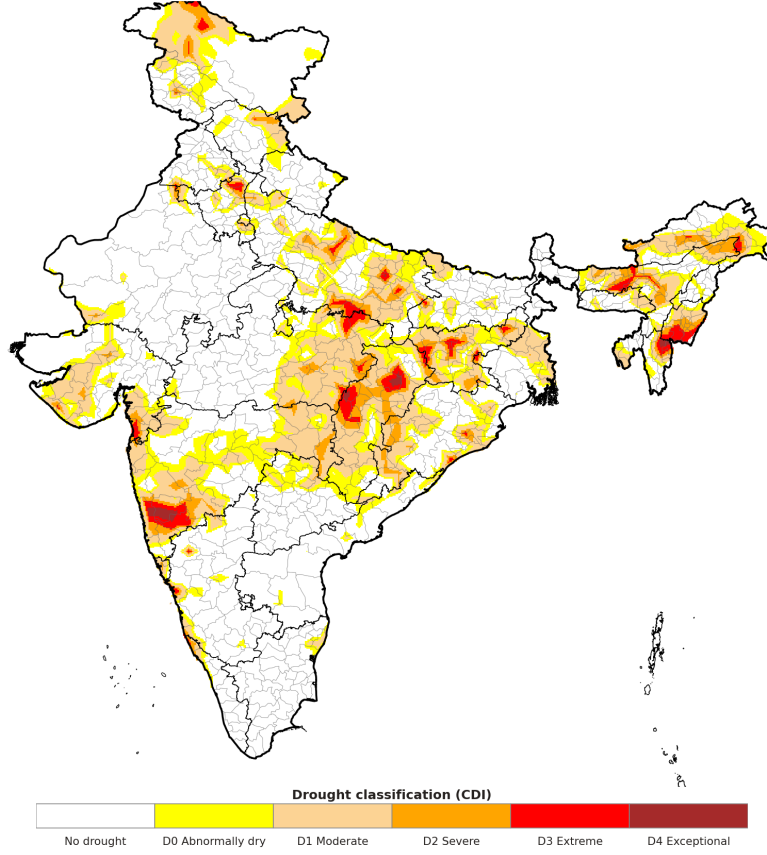
Combined Drought Index (CDI) for the week ending July 1, 2026.
