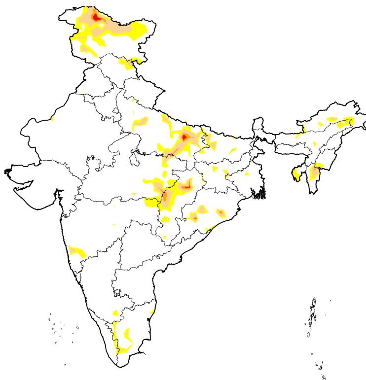
Combined Drought Index (CDI) for the week ending April 15, 2026.
