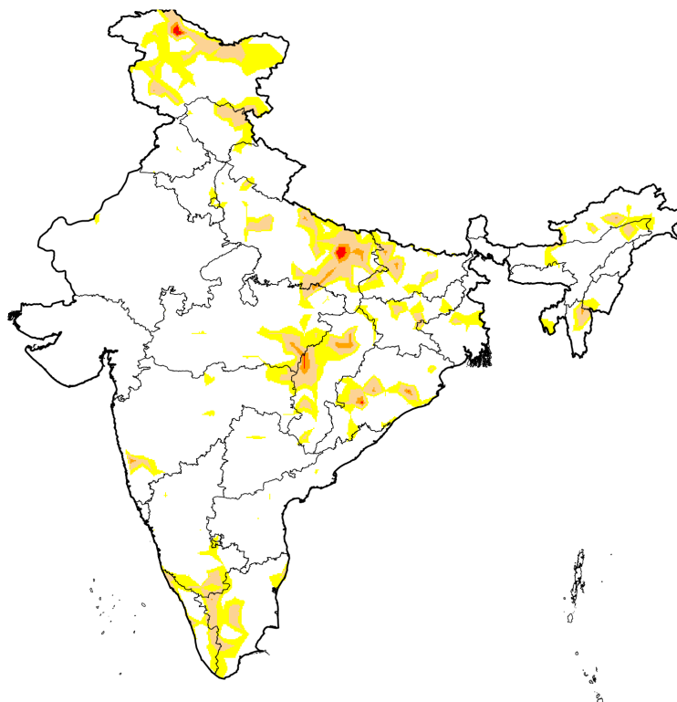
Combined Drought Index (CDI) for the week ending April 29, 2026.
