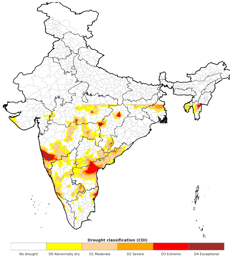
Combined Drought Index (CDI) for the week ending August 19, 2026.
