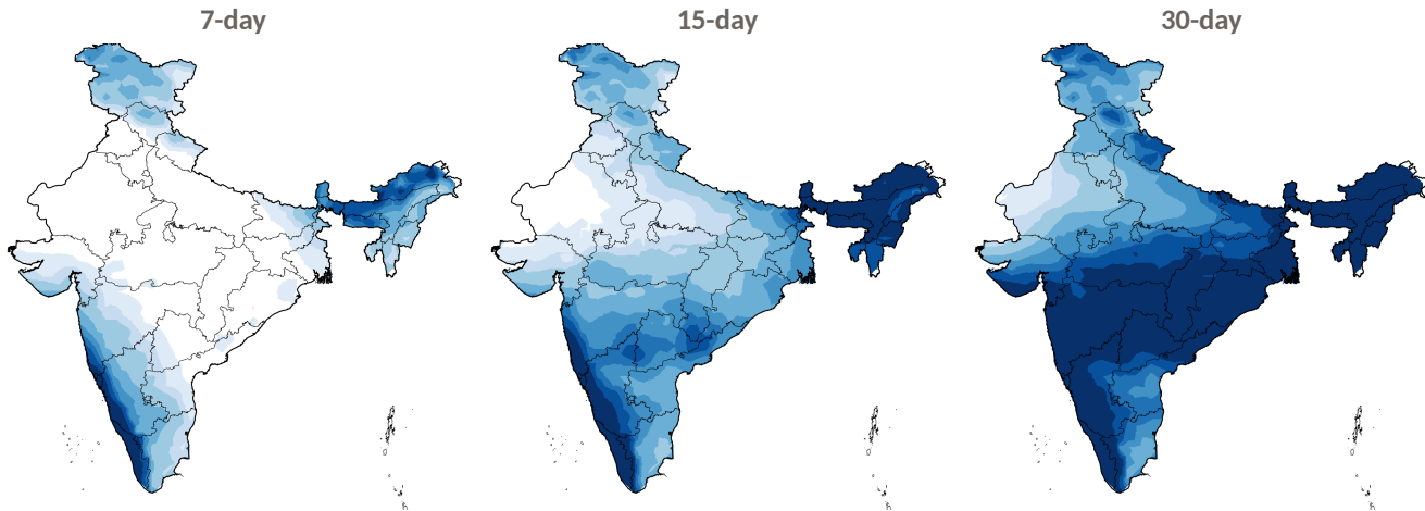
Forecast rainfall for the 7-, 15- and 30-day horizons, initialized May 20, 2026.
