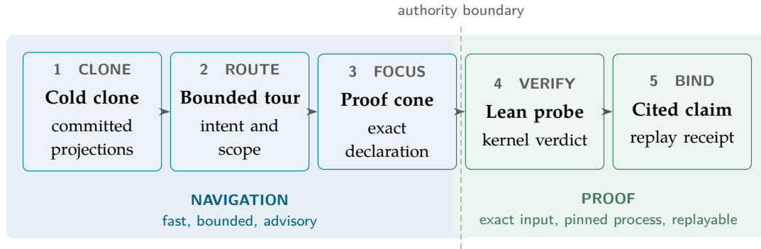
Figure 2: The shortest path from first contact to an authoritative receipt. The agent chooses the route; the pinned Lean process supplies the verdict.
