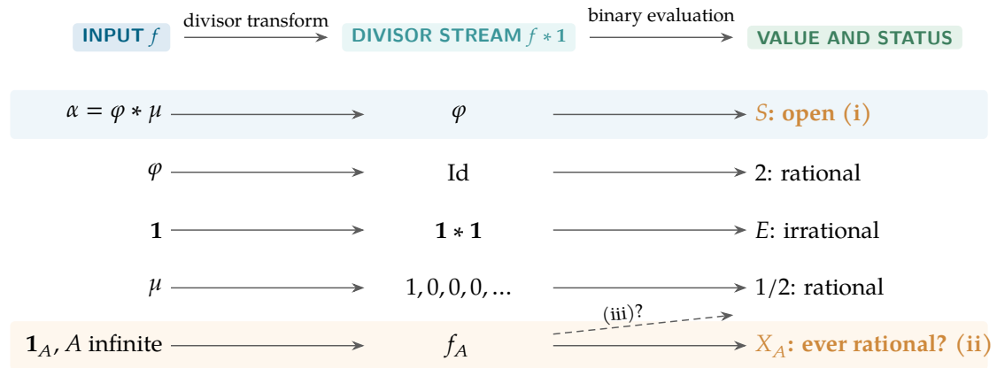
Figure 1: The divisor transform and its five benchmark inputs. The shaded rows are the open questions: (i) asks for the status of the single value S , while (ii) asks whether an infinite Boolean input can have any rational image. The dashed arrow marks (iii), the narrower question of whether such an input can reach the calibrated value 1/2 . The remaining three rows calibrate the transform with known rational and irrational values.
