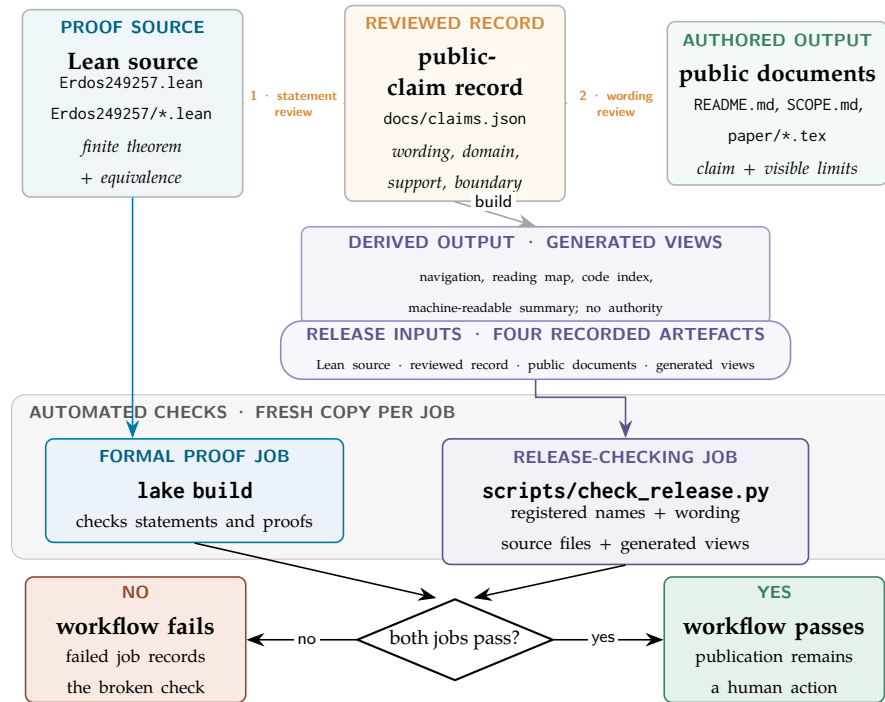
Figure 2: Configured checks for one saved change. Amber dashed connectors are human review; solid connectors are recorded inputs and automated checks. Lean checks the formal proof, while the release job checks registered names, wording, source files, and generated views. A passing workflow still leaves publication as a human action. Neither job interprets unrestricted prose.
