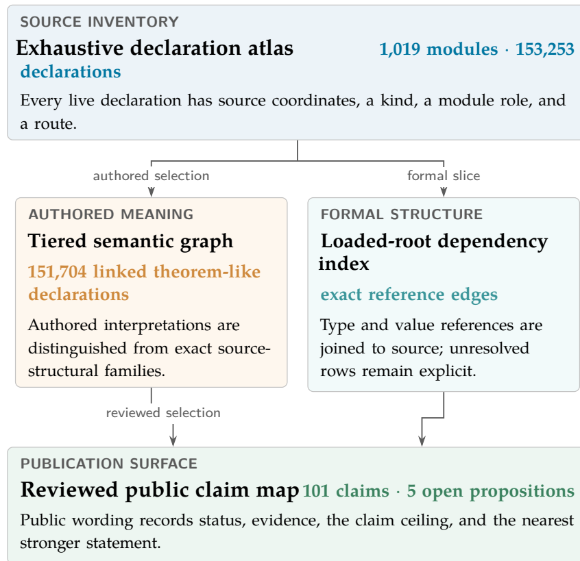
Figure 1: The navigation layers. The dependency index and semantic graph are different partial views of the exhaustive atlas; neither is presented as a complete interpretation.
