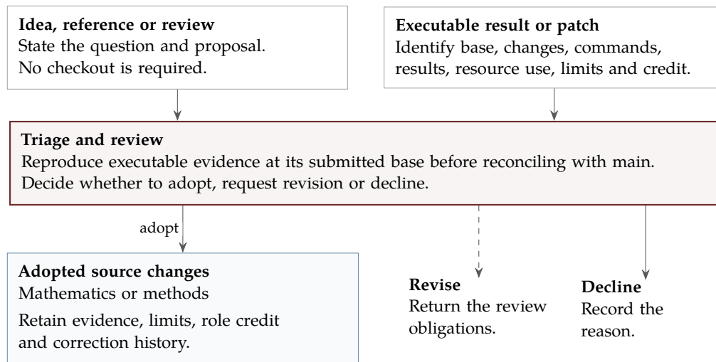
Figure 6: Two entry routes and three dispositions. Adopted work includes mathematics and methods. Only explicitly entered returns become journal events; adoption establishes neither independent review nor wider acceptance.
