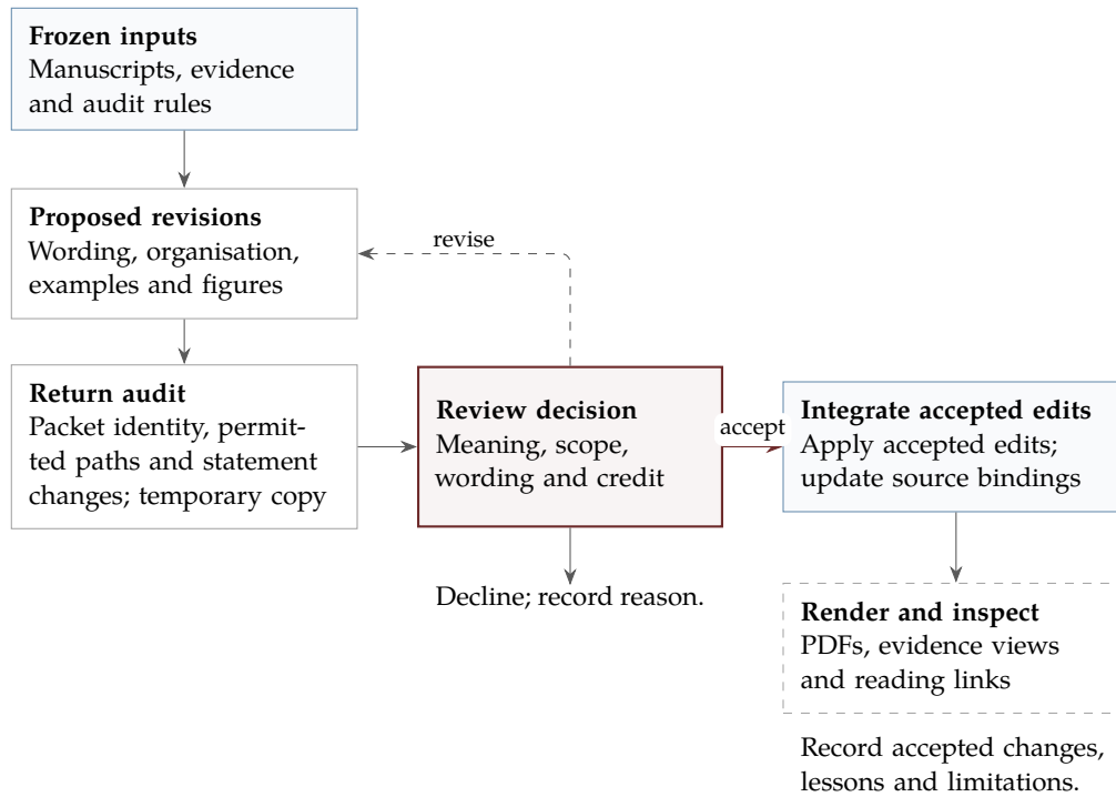
Figure 5: Only accepted edits enter live sources. The return audit neither applies edits nor executes returned programs. Review may request revision or decline; one agent may perform several responsibilities.
