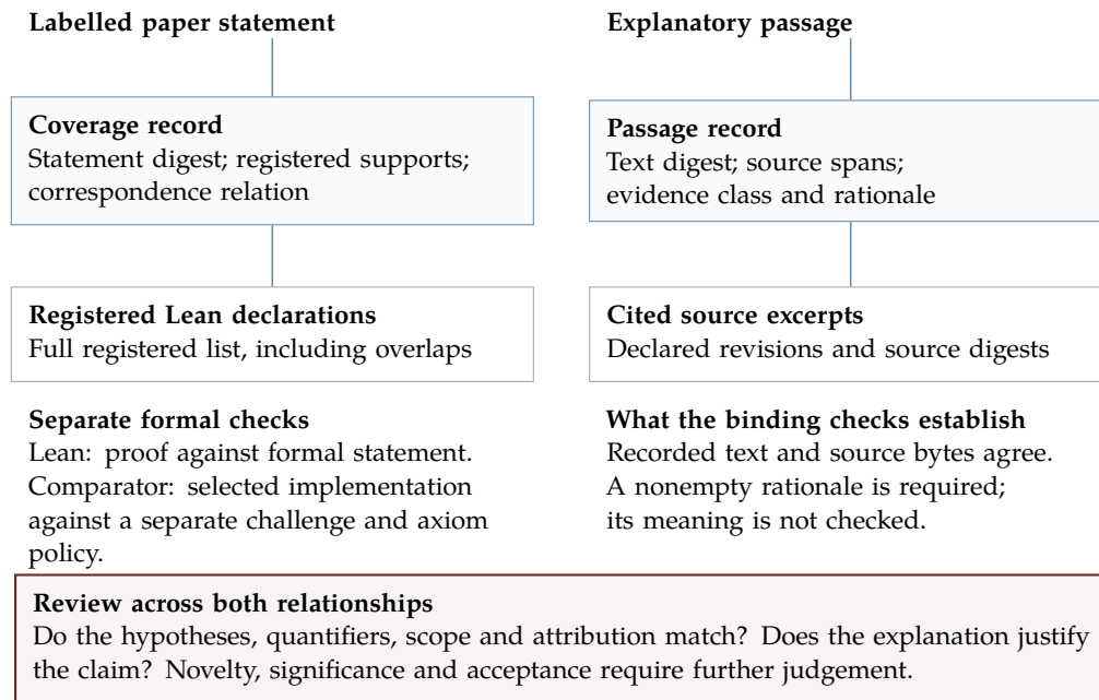
Figure 4: Two correspondence records. Lines are recorded links, not implications. Binding and formal checks do not establish the paper’s intended meaning. Review responsibilities do not imply independent review.
