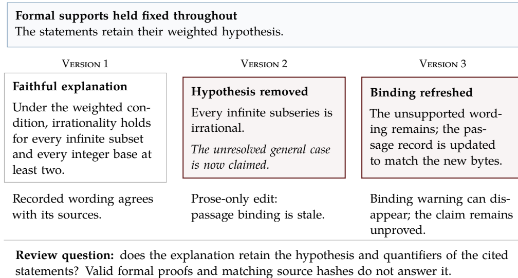
Figure 3: Hypothesis loss with unchanged formal supports. Rebinding can restore byte consistency while leaving the overclaim intact. This is an illustration, not a new test or historical edit 8.
