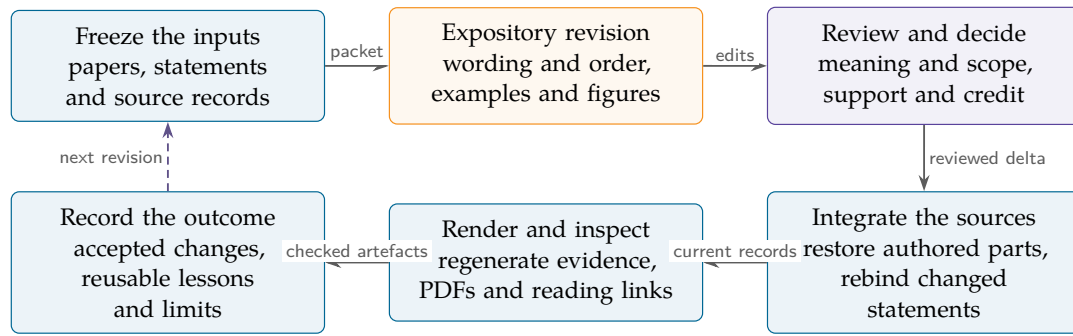
Figure 5: An exposition assignment returns focused source changes and optional figures for review; the stages describe responsibilities, not necessarily different people, and integration, rendering and the recorded outcome remain separate.
