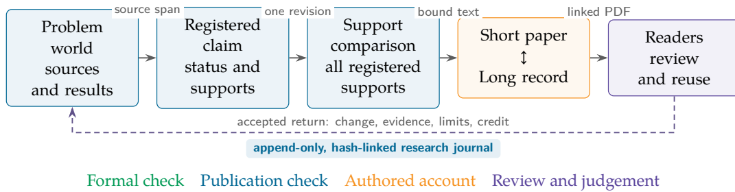
Figure 1: The life of one claim: arrows name the objects exchanged, and the support comparison checks the complete recorded set without executing a new formal proof; the short and long accounts remain linked.
