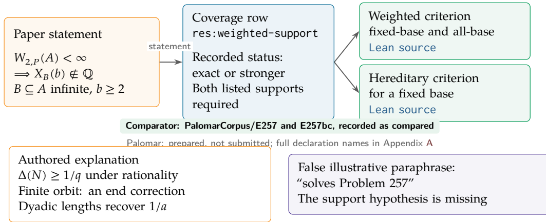
Figure 3: Both registered supports are required for the coverage row, while the authored explanation must justify the hypothesis and its use; omitting that hypothesis can change the claim without breaking either link, as the illustrative paraphrase shows (a different example from historical edit 8 in Table 1).
