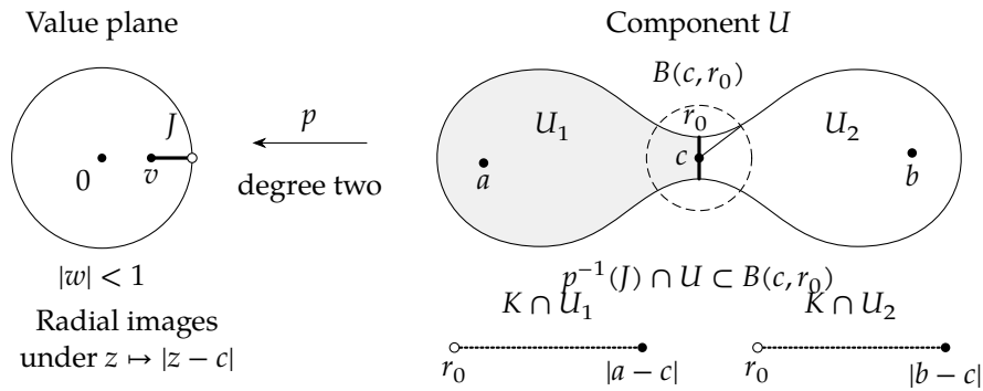
Figure 1: The slit and its preimage in Lemma 2.1. The component and radii are schematic, with both zeros drawn outside the small disc. Connectedness forces the radial image on each sheet to contain the indicated interval. The two 1-Lipschitz projections give the lower bound |a - c| + |b - c| - 2r_0 . The dotted intervals are radial images, not paths in U ; no parametrisation of K is assumed.
