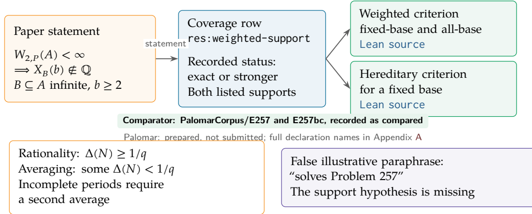
Figure 3: Both arrows out of the coverage row represent registered supports, with recorded status distinguished from a fresh check; the false paraphrase illustrates a meaning error separate from historical edit 8 in Table 1.
