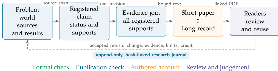
Figure 1: The life of one claim: arrows name the objects exchanged, and the blue evidence join checks the recorded support relation rather than executing a new formal proof; the short and long accounts remain linked.
