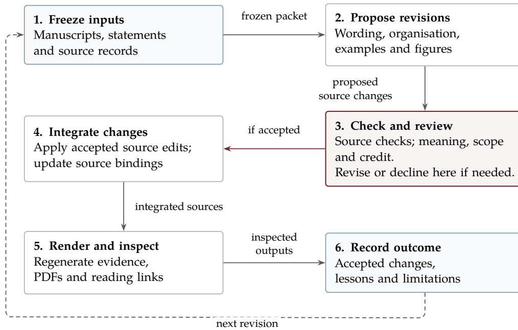
Figure 4: Exposition workflow in numbered order, with exchanged objects labelled. Step 3 may request revision or decline a proposal; only accepted changes reach integration. These are responsibilities, which one agent may perform. Rendering and inspection remain separate from source checks.
