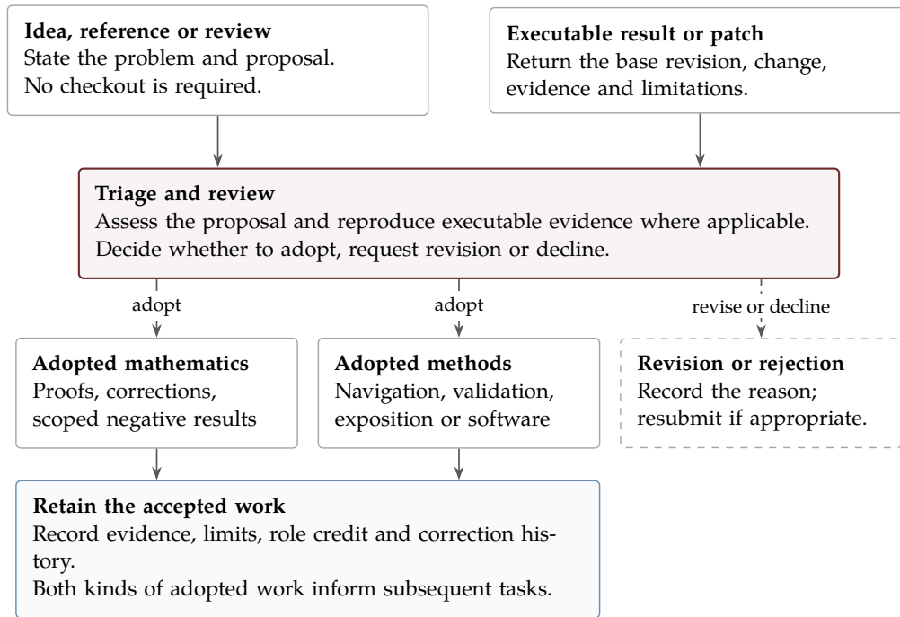
Figure 5: Two entry routes and three possible review outcomes. Repository adoption applies to mathematical and methodological contributions; it establishes neither independent review nor acceptance by the wider mathematical community.
