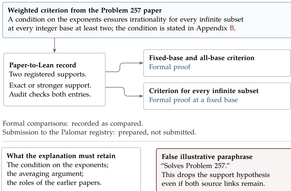
Figure 6: The arrows show recorded support links, not proof dependencies. The audit checks both listed supports even where their mathematical roles overlap. The support hypothesis still needs explanation. The false paraphrase is illustrative, distinct from historical edit 8 in Table 1.
