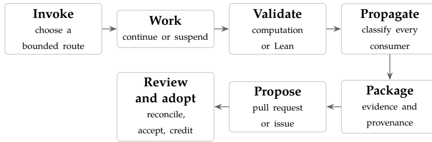
Figure 2: The clone-local job lifecycle. Closure means that the present delta has evidence and dispositions; it does not mean that the open problem is solved.
