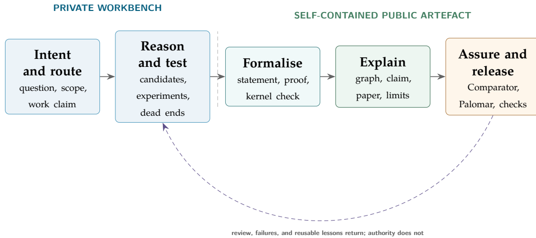
Figure 1: The end-to-end architecture. The dashed vertical line is a release boundary, not a network connection: the public repository must remain usable without the private workbench.
