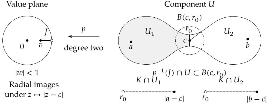
Figure 1: The slit and its preimage in Lemma 2.1. The component and radii are schematic, with both zeros outside the small disc. Connectedness forces the radial image on each sheet to contain the dotted interval. These intervals are displayed separately, although they may overlap as subsets of the real line. The two measure contributions add because U_1 and U_2 are disjoint in the plane, giving |a - c| + |b - c| - 2r_0 . The dotted intervals are not paths in U .
