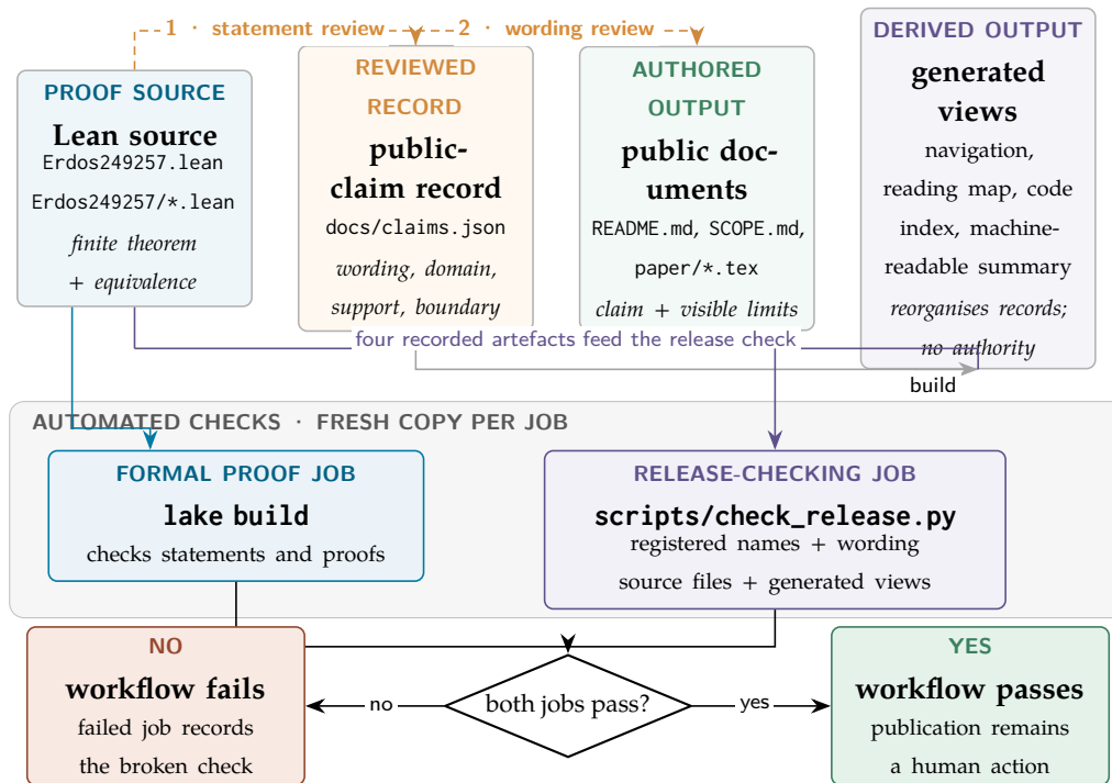
Figure 2: Configured checks for one saved change. Amber dashed connectors are human review; solid connectors are recorded inputs and automated checks. Lean checks the formal proof, while the release job checks registered names, wording, source files, and generated views. A passing workflow still leaves publication as a human action. Neither job interprets unrestricted prose.
