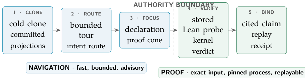
Figure 2: The shortest path from first contact to an authoritative receipt. The agent chooses the route; the pinned Lean process supplies the verdict.
