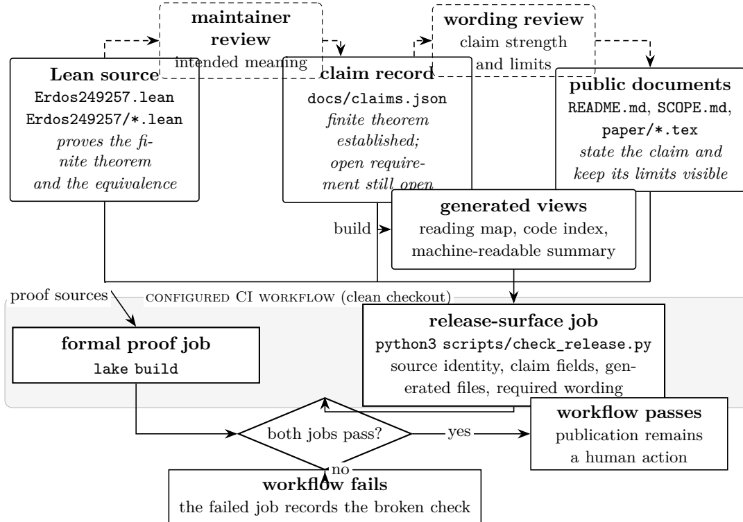
Figure 1: The configured checks for one revision. Dashed elements are human judgements; solid elements are files and programs. Three relations of different kinds meet here. Lean establishes the proof relation : the source proves the stated theorems. Maintainer review asserts the semantic relation : the recorded wording describes those theorems within stated limits. The release job checks persistence relations : recorded names, wording, identities, and generated files still agree. Continuous integration reruns the first and third; nothing performs the second mechanically, and neither job reads unrestricted prose or adds authority. In the worked example the protected object is the recorded boundary between the finite theorem and the open requirement.
