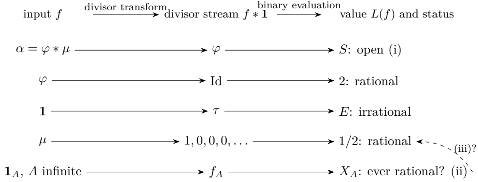
Figure 1: The one transform behind the paper, with the statuses of Section 3. Labels (i)–(iii) are the three questions of Section 6.1: #249 fixes the top input and asks about the single image point S ; universal #257 restricts the domain to indicators of infinite supports and asks whether its image ever meets \mathbb{Q} ; the half-value route fixes the value 1/2 , reached by the signed Möbius input through the stream 1, 0, 0, 0, \dots , and asks whether an infinite Boolean input reaches it as well. The figure organises statements proved in Sections 3–4 and Appendix B; it asserts nothing further.
