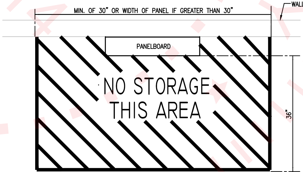
TYPICAL CLEARANCE AT ELECTRICAL PANELS NOT TO SCALE
