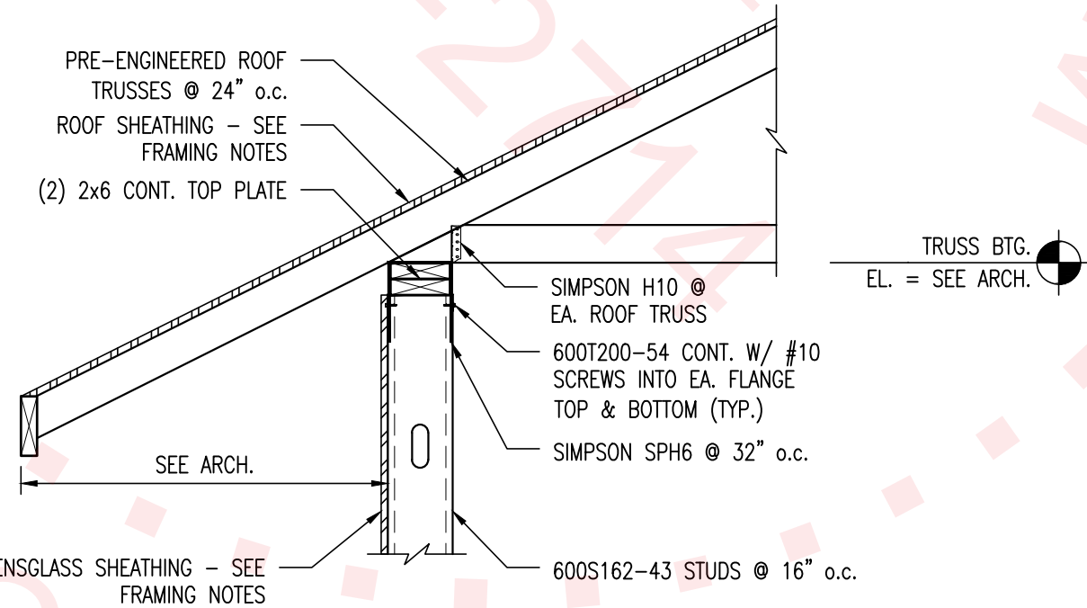
WALL BEARING DETAIL SCALE: ¾" = 1'-0"
