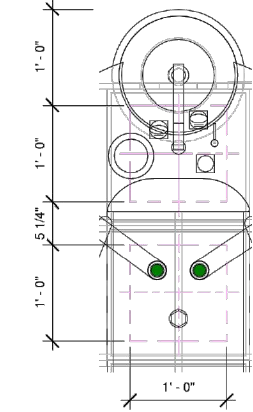
④ ENLARGED CENTRAL CABINET UTILITY ITEM #21 1" = 1'-0"
