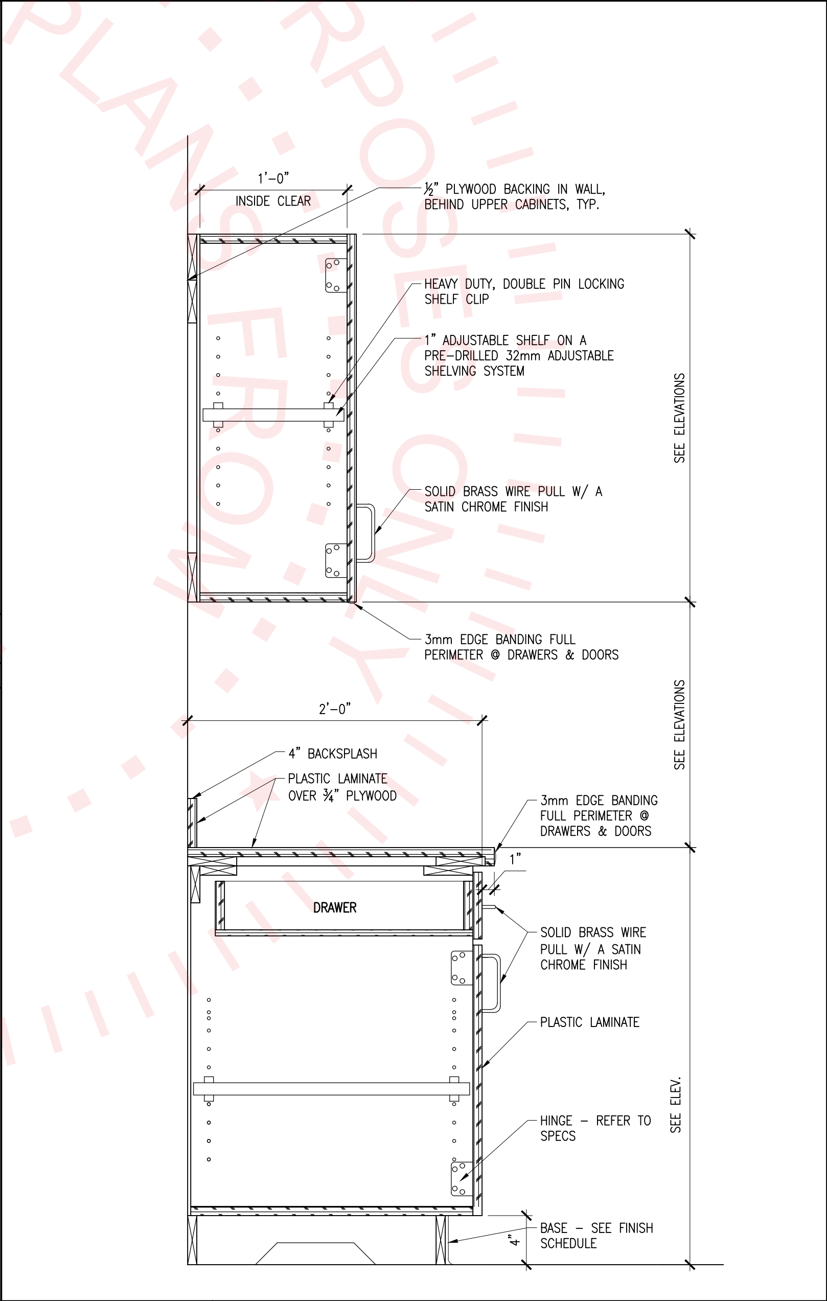
A3 TYPICAL CASEWORK SECTION SCALE: 1-1/2" = 1'-0"
