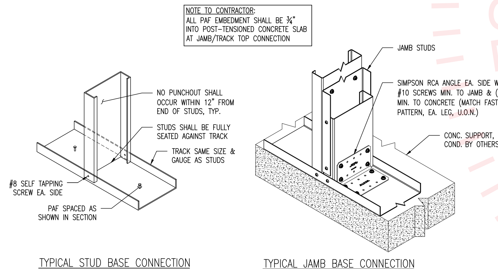
TYPICAL STUD BASE CONNECTION
