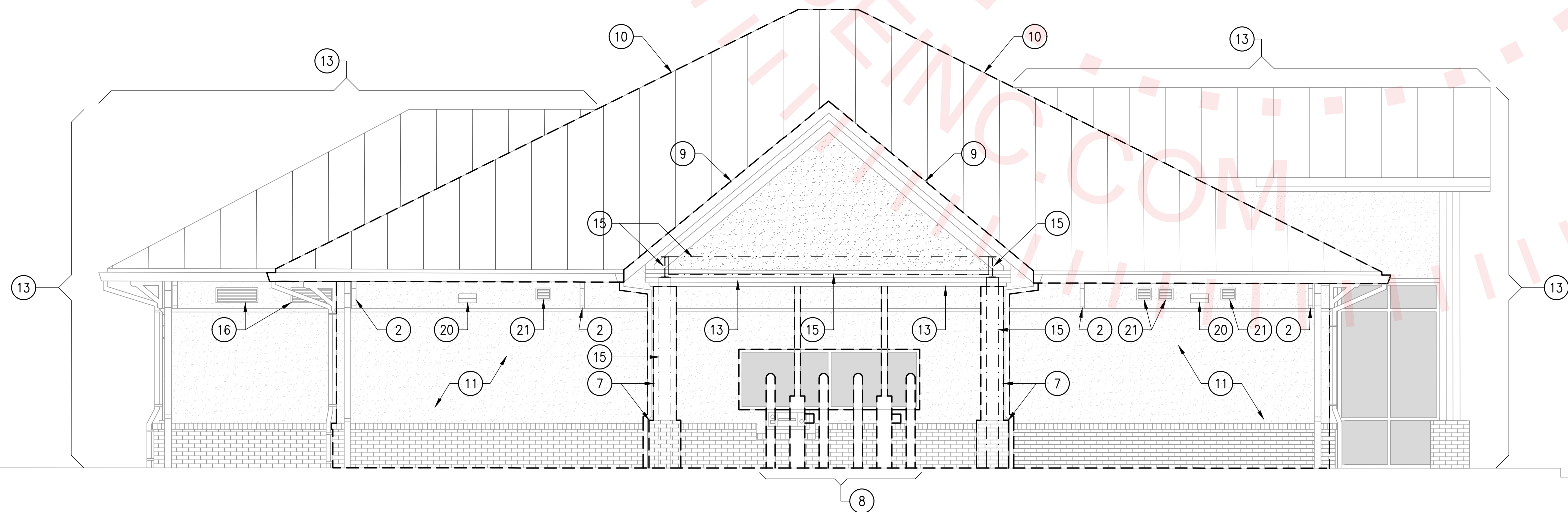
A1 WEST ELEVATION
