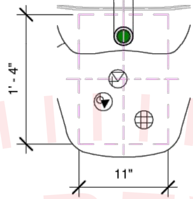
② ENLARGED CHAIR UTILITY ITEM #1 1" = 1'-0"
