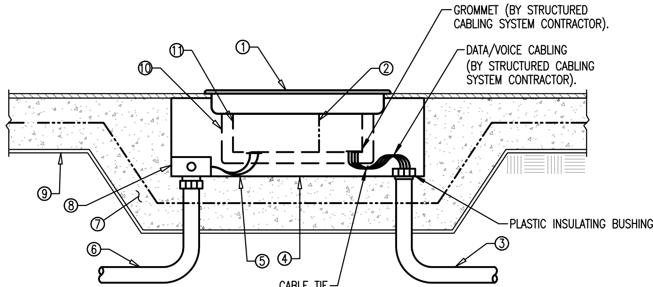
FLOOR BOX INSTALLATION DETAIL
