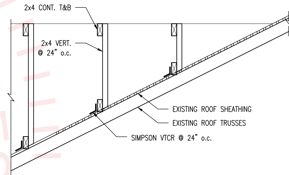
OVERFRAMING DETAIL SCALE: ¾" = 1'-0"
