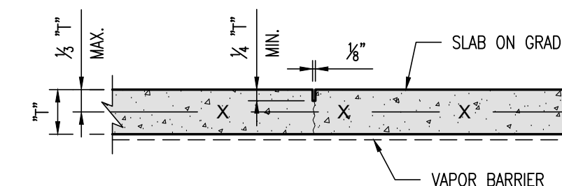
SAWCUT CONTROL JOINT (SCJ) NOTE: SAWCUT SLAB WITHIN 12 HOURS OF POURING SLAB
