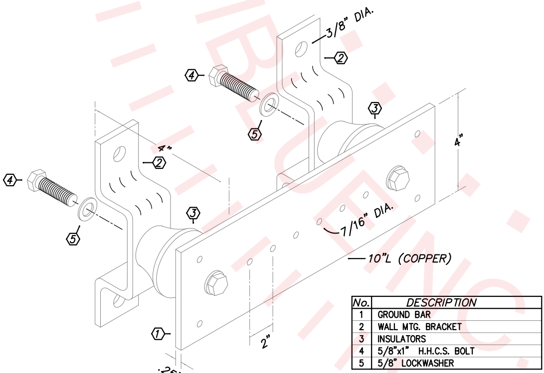
INSULATED GROUNDING BUSBAR DETAIL NOT TO SCALE
