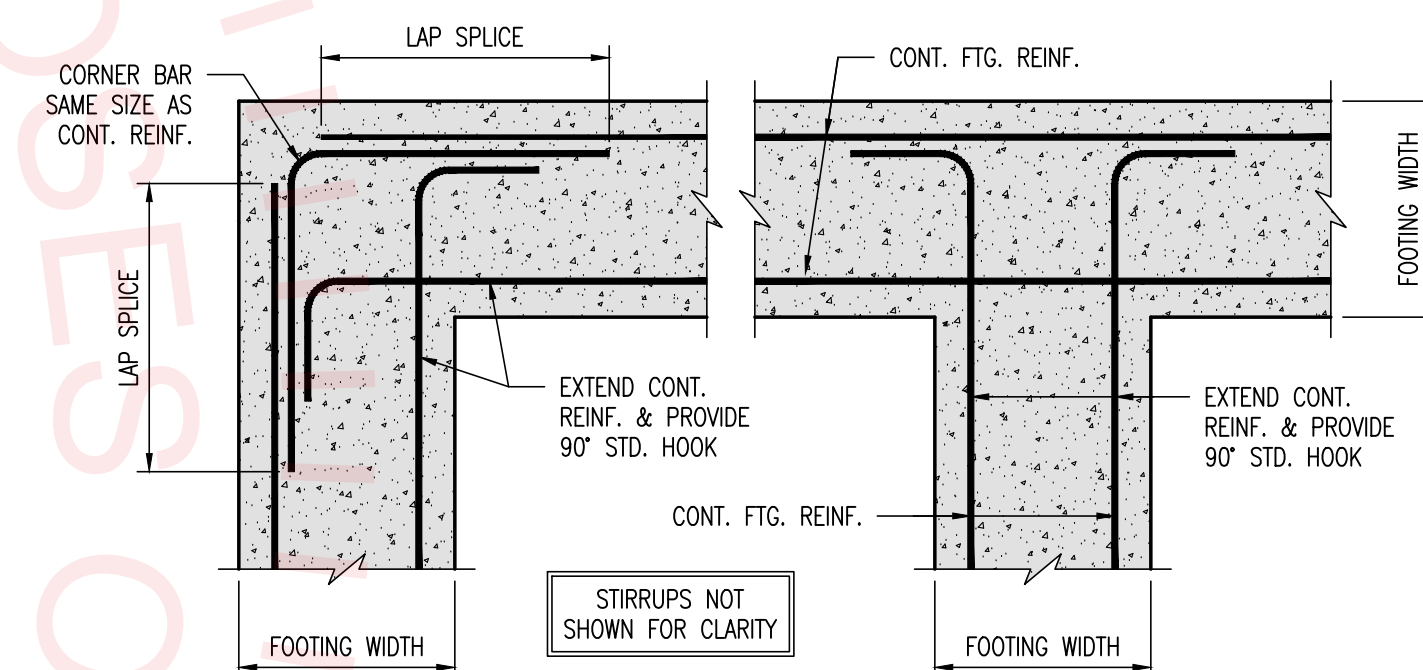
TYP. FOOTING INTERSECTION DETAIL (F) SCALE: \frac{3}{4}" = 1'-0" S20
