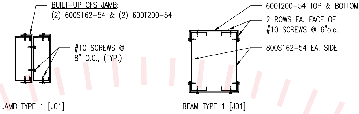
BUILT-UP MEMBER DETAIL NO SCALE
