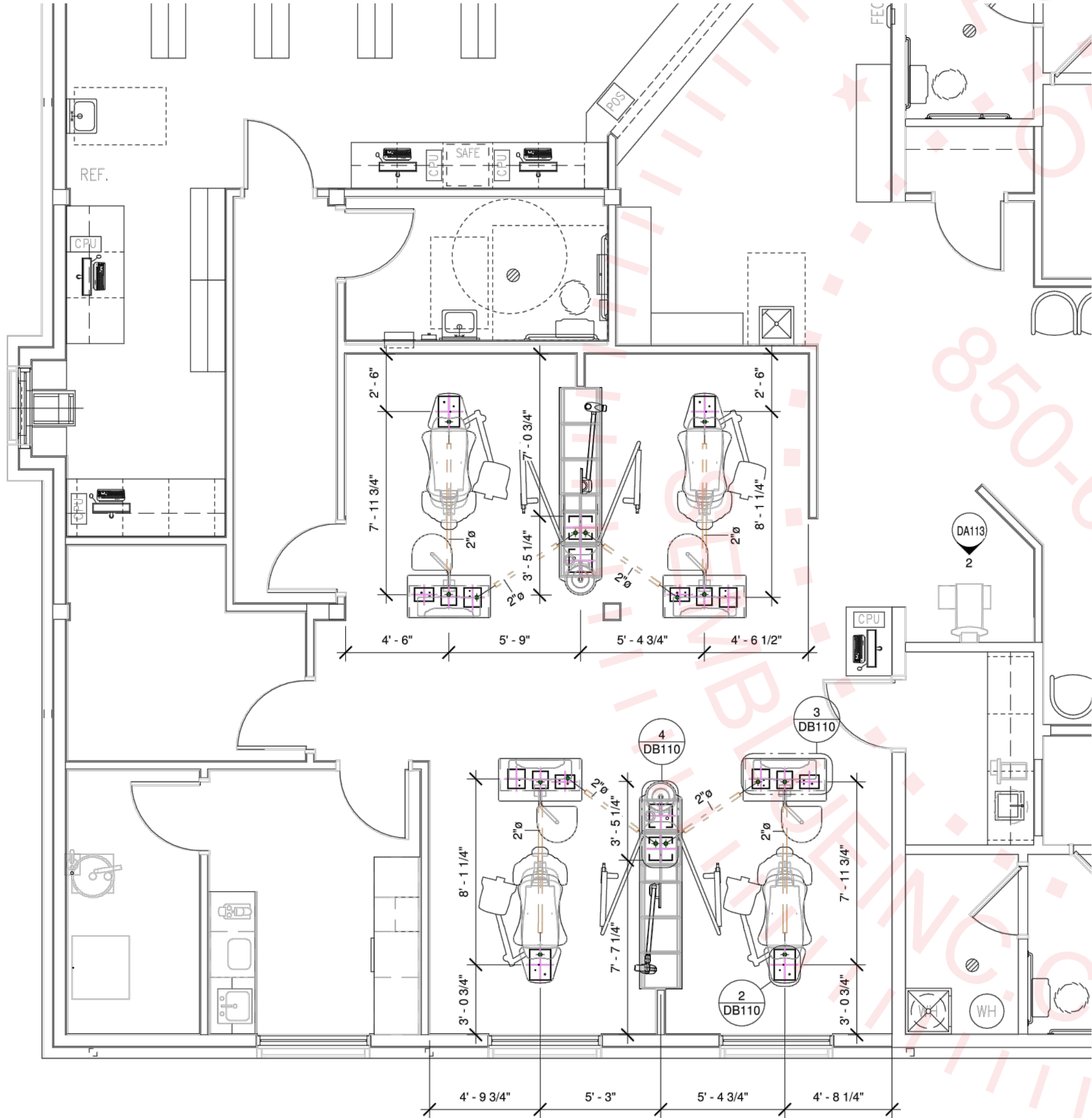
① LVL 1 UNDER FLOOR UTILITY PLAN 1/4" = 1'-0"
