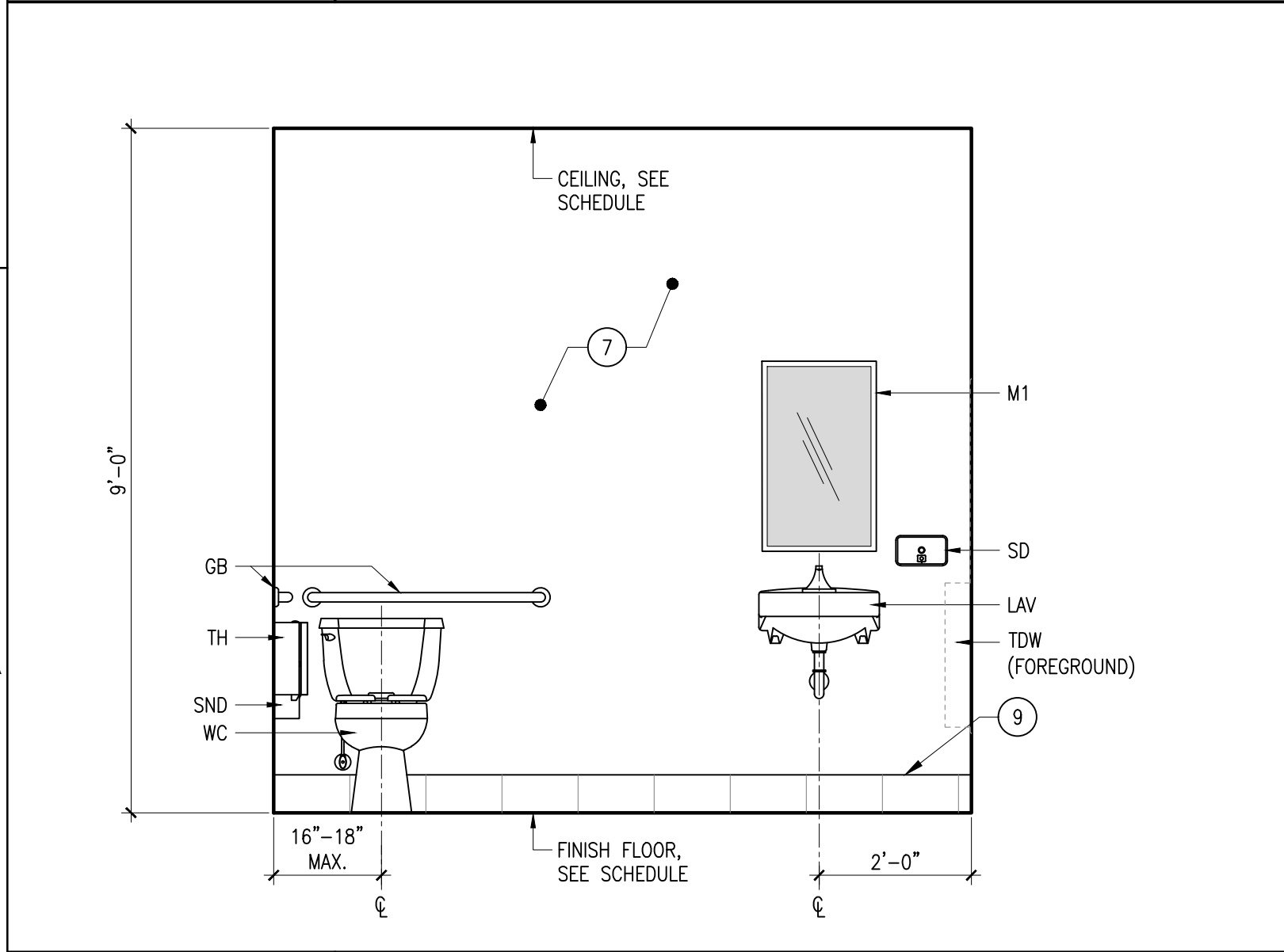
A1 INTERIOR ELEVATION SCALE: 1/2" = 1'-0" TOILET #108
