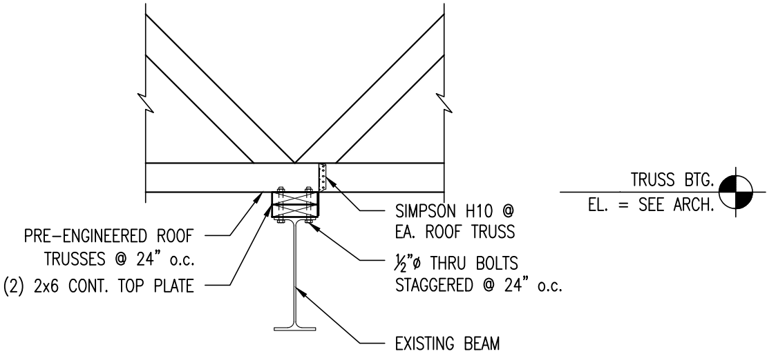
INTERIOR BEAM BEARING DETAIL SCALE: ¾" = 1'-0"
