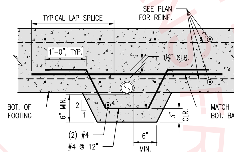
PIPE CONFLICTS WITH FOOTING REINFORCEMENT
