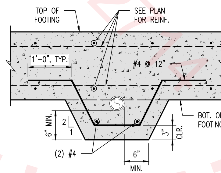
PIPE CONFLICTS WITH FOOTING REINFORCEMENT
