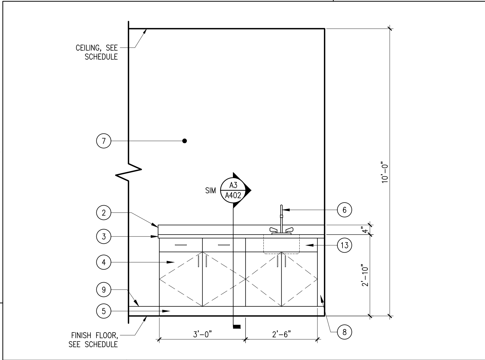
C1 INTERIOR ELEVATION SCALE: 1/2" = 1'-0" TYPICAL EXAM ROOM CASEWORK
