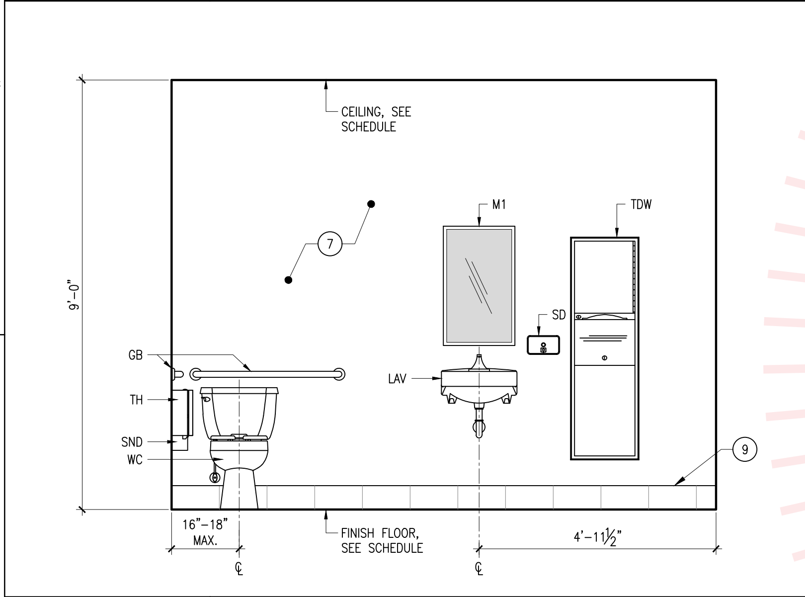
B1 INTERIOR ELEVATION SCALE: 1/2" = 1'-0" TOILET #135
