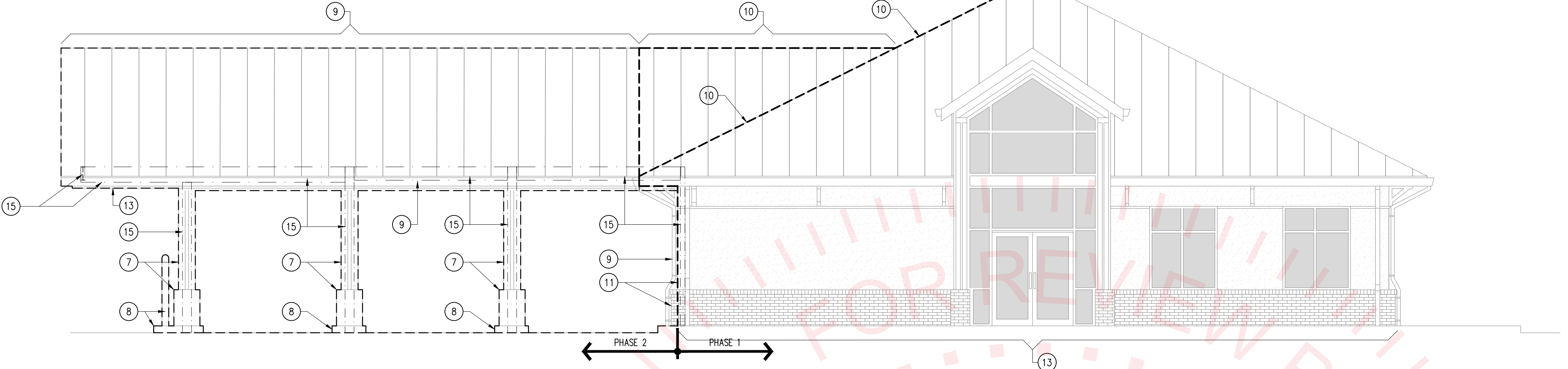
C1 | SOUTH ELEVATION
