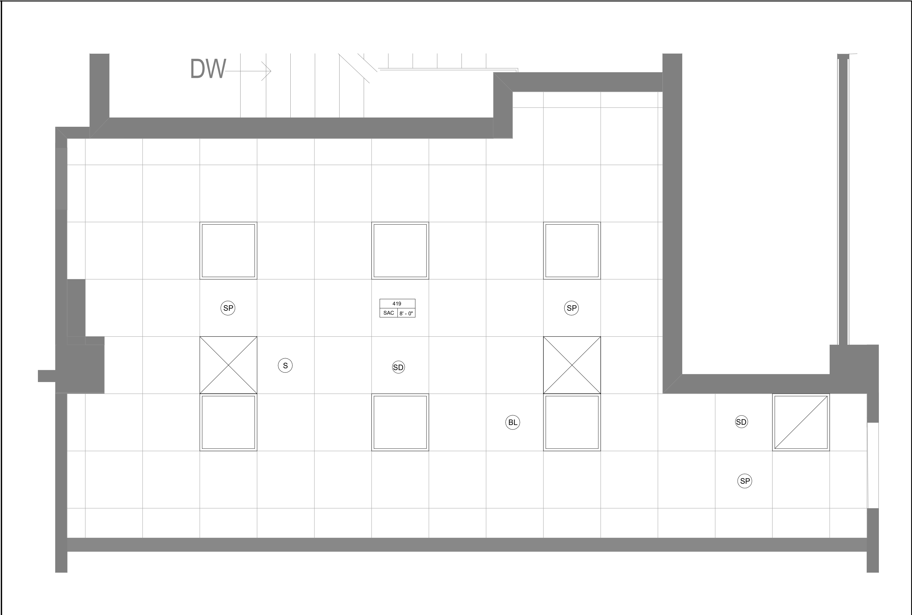
1 EXISTING REFLECTED CEILING PLAN LEVEL 4 - ROOM 419 EX2.1 1/2" = 1'-0"
