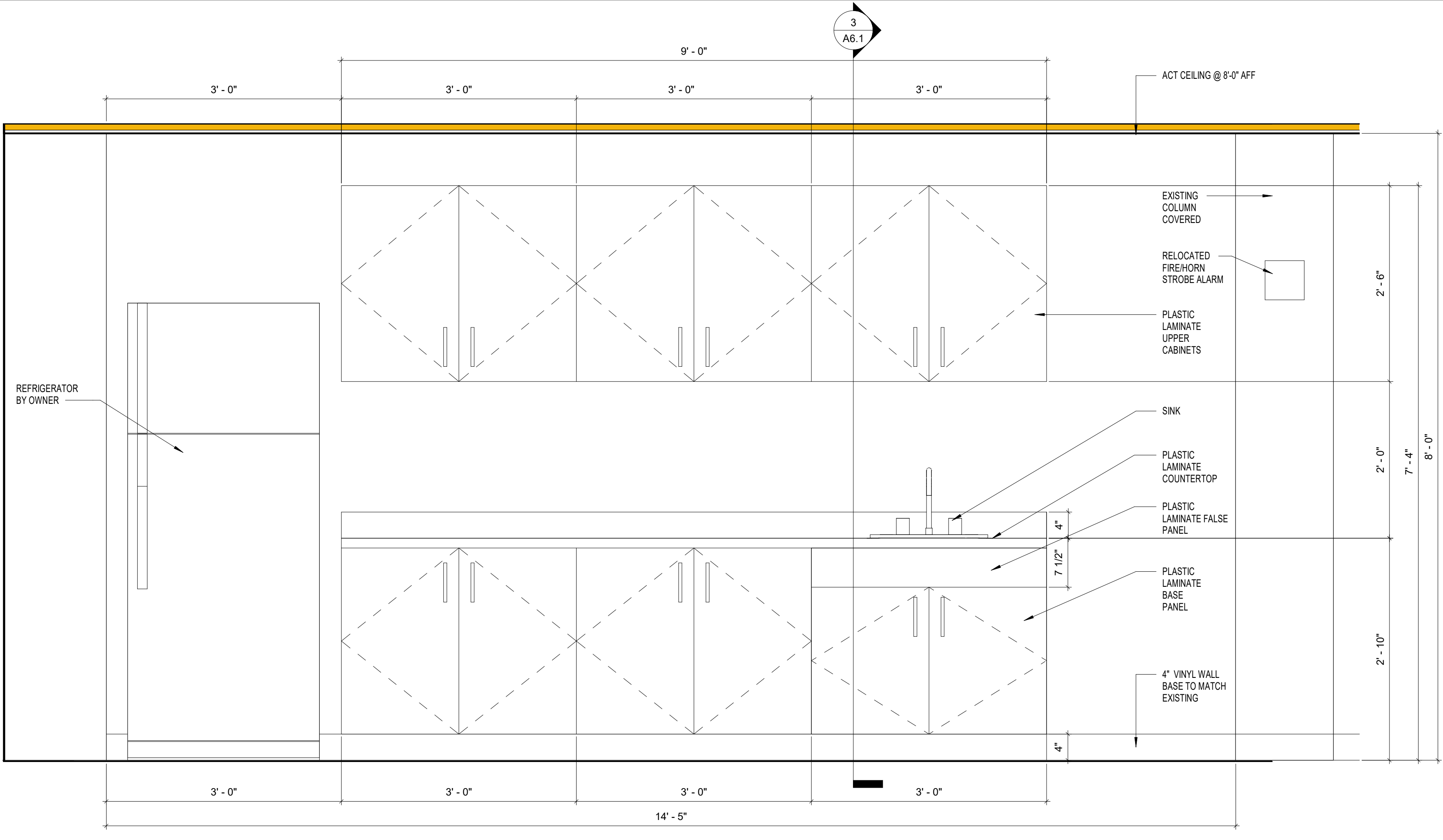
2 CONFERENCE MILLWORK ELEV. A6.1 1" = 1'-0"
