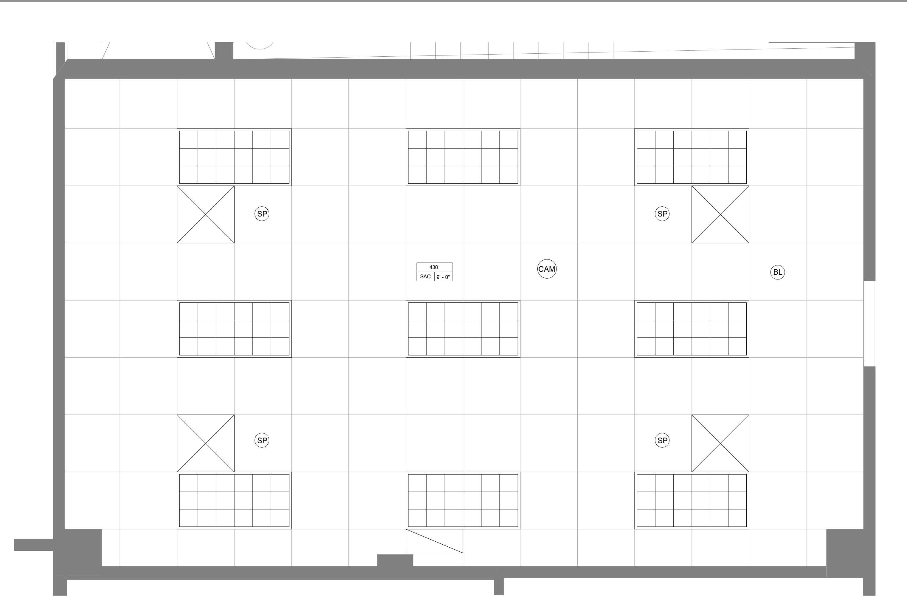
3 EXISTING REFLECTED CEILING PLAN LEVEL 4 - ROOM 430 EX2.1 1/2" = 1'-0"
