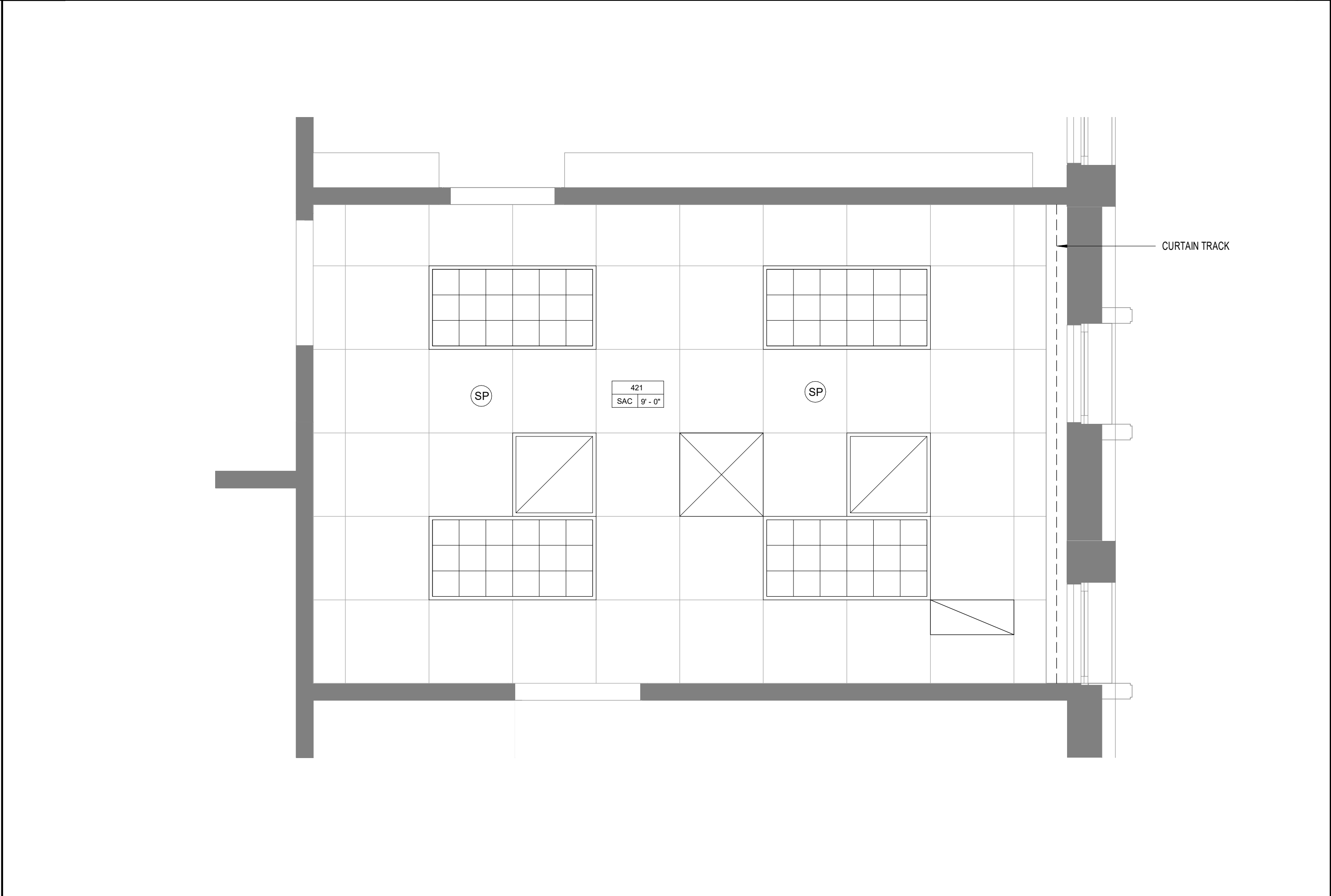
2 EXISTING REFLECTED CEILING PLAN LEVEL 4 - ROOM 421 EX2.1 1/2" = 1'-0"
