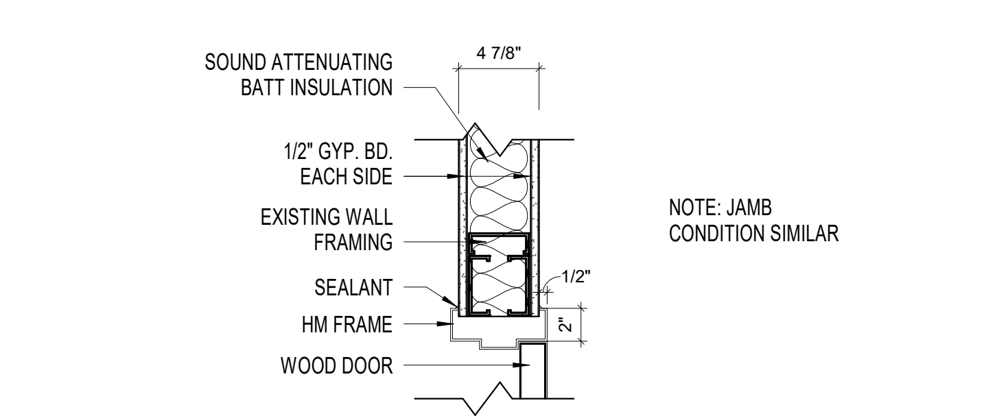
4 HEAD DETAIL A6.1 1 1/2" = 1'-0"
