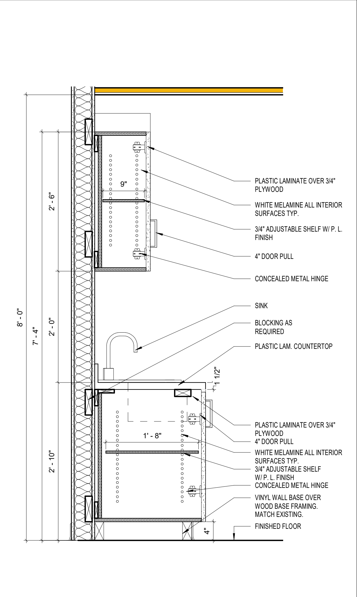
3 CONF. CASEWORK SECTION A6.1 1" = 1'-0"
