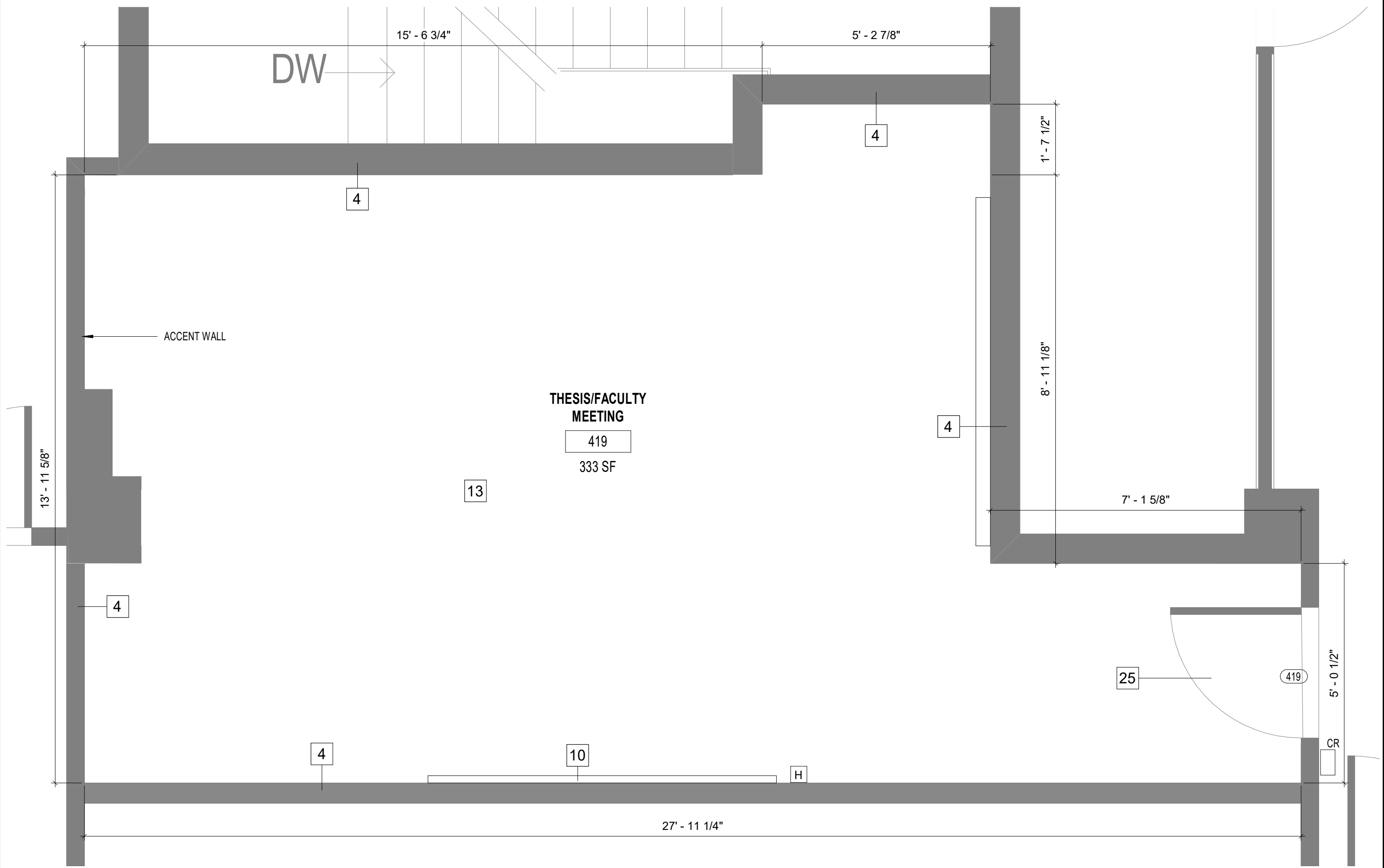
1 NEW LEVEL 4 - ROOM 419 A1.1 1/2" = 1'-0"
