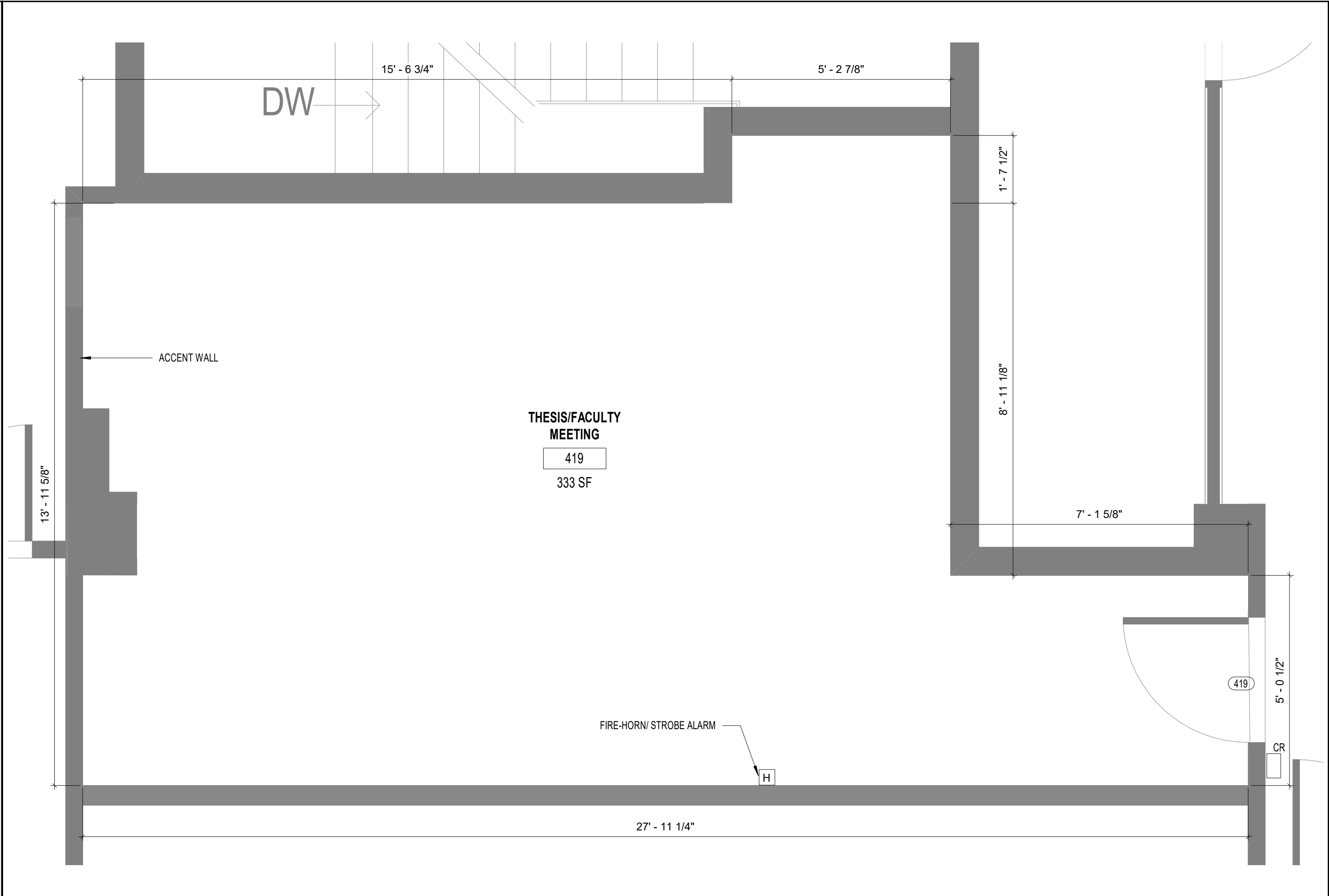
1 EXISTING LEVEL 4 - ROOM 419 EX1.2 1/2" = 1'-0"
