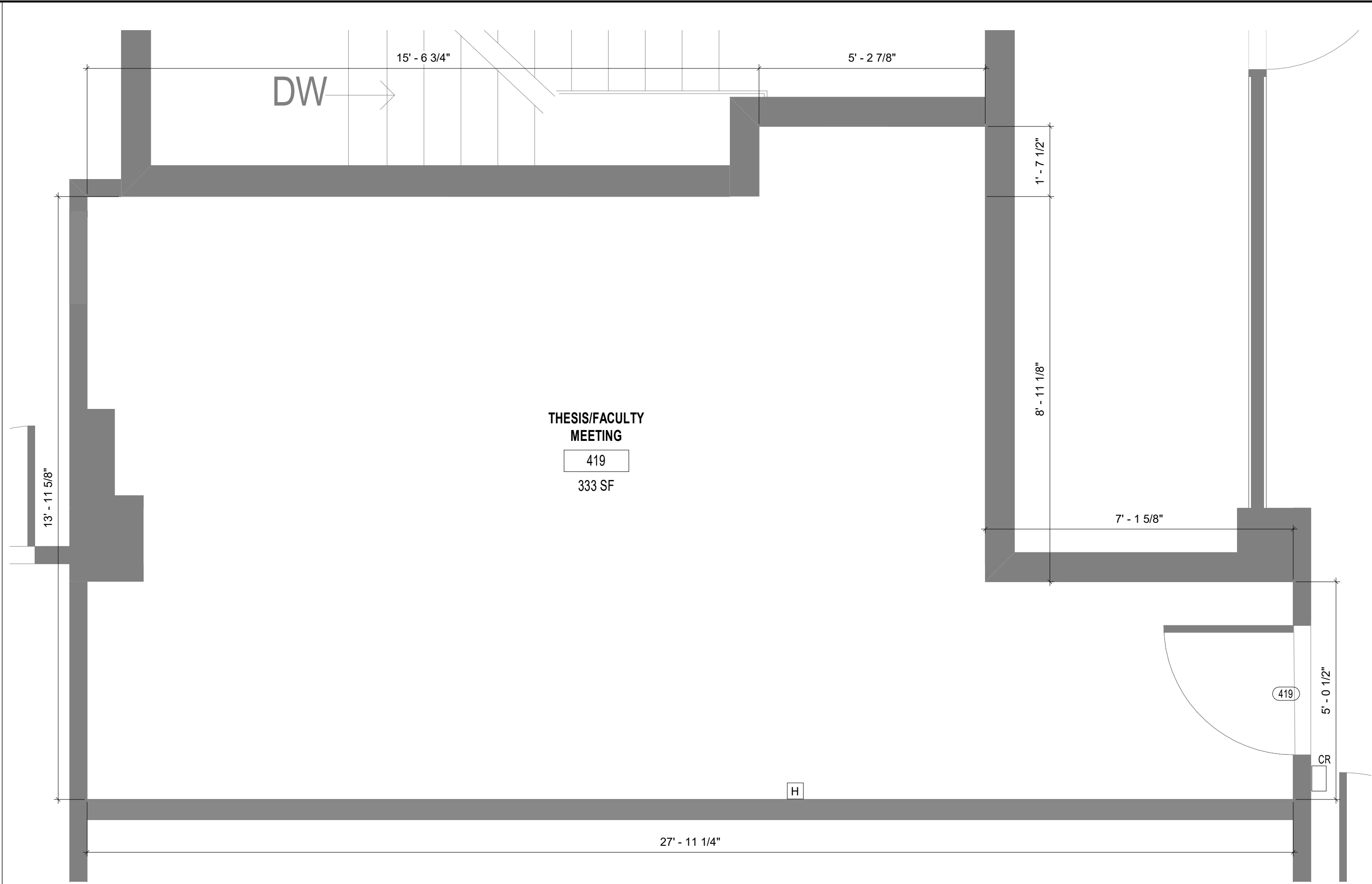
1 DEMO LEVEL 4 - ROOM 419 D1.1 1/2" = 1'-0"
