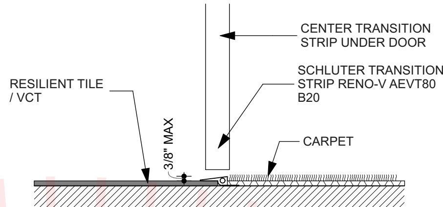
5 A-601 RESILIENT TILE / VCT TO CARPET SCALE: 3" = 1'-0"
