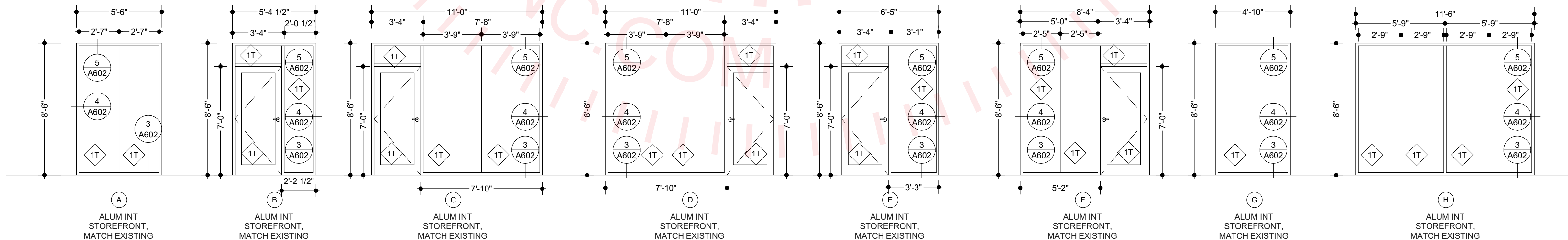
1 A-602 Window Elevations SCALE: 1/4" = 1'-0"
