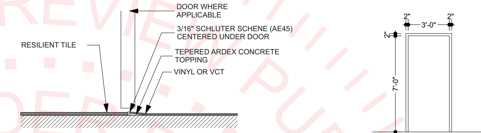
4 A-601 RESILIENT TILE TO VINYL / VCT SCALE: 3" = 1'-0"
