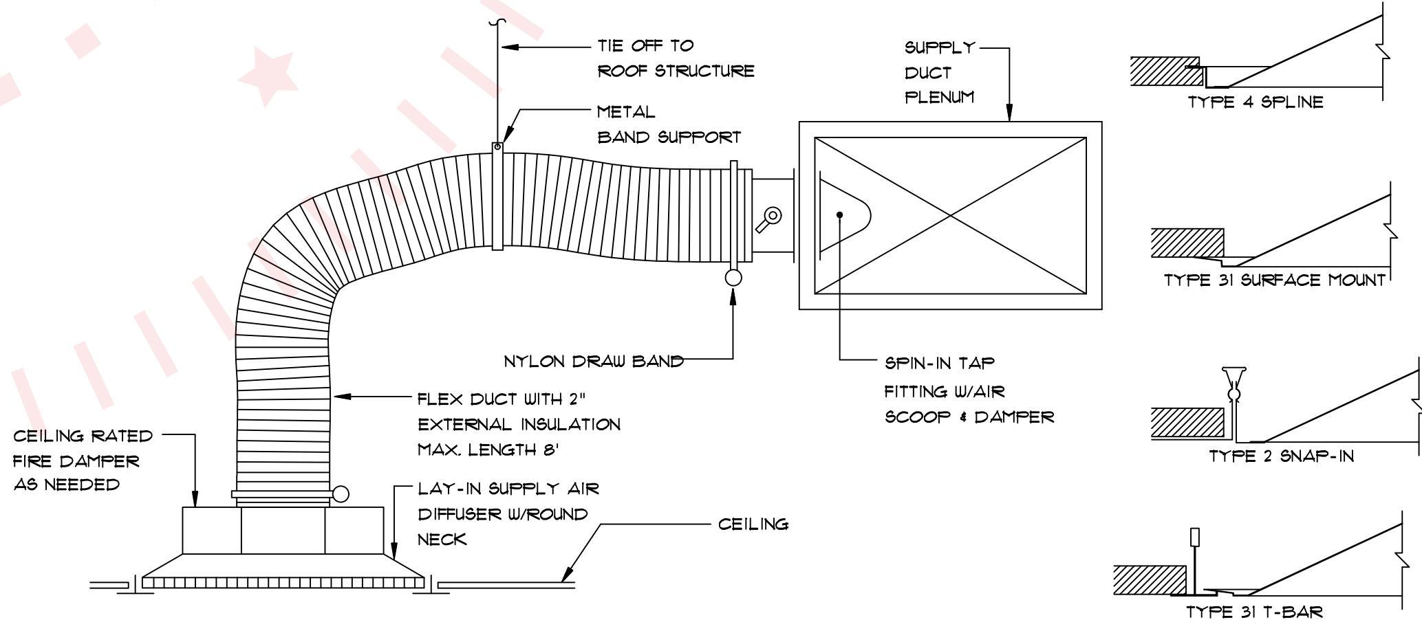
SUPPLY AIR DIFFUSER DETAIL N.T.S.
