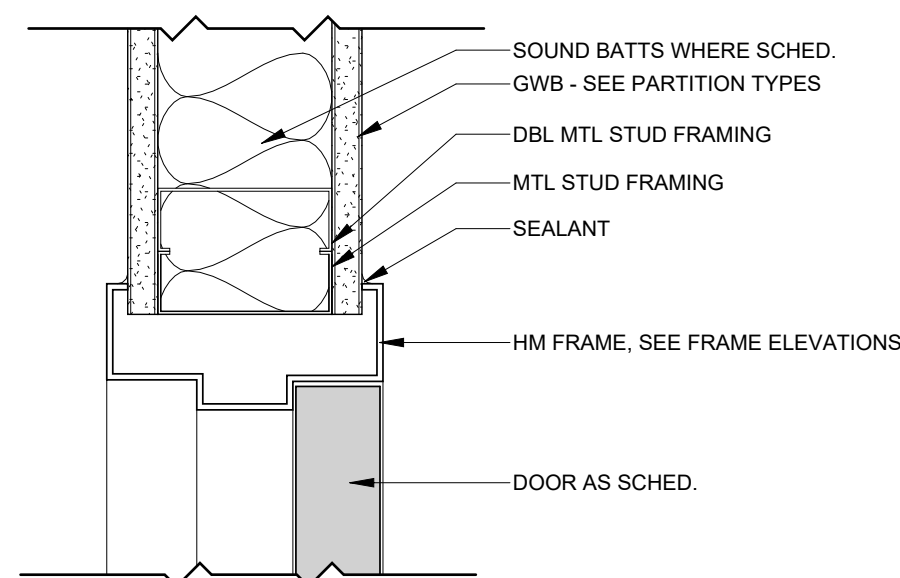
1 Interior HM Door Head 3" = 1' - 0"
