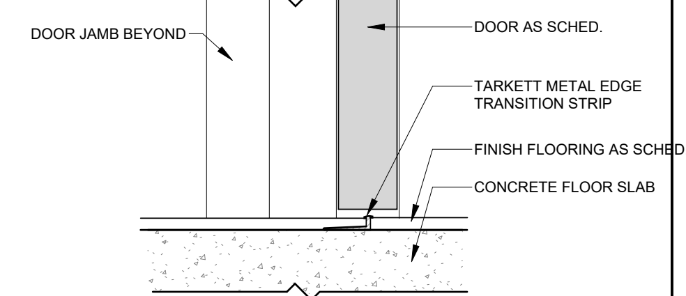
15 Interior HM Door Threshold w/ Metal Edge Transition 3" = 1' - 0"
