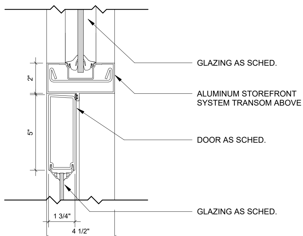
6 Interior Storefront Transom & Door Head 3" = 1' - 0"
