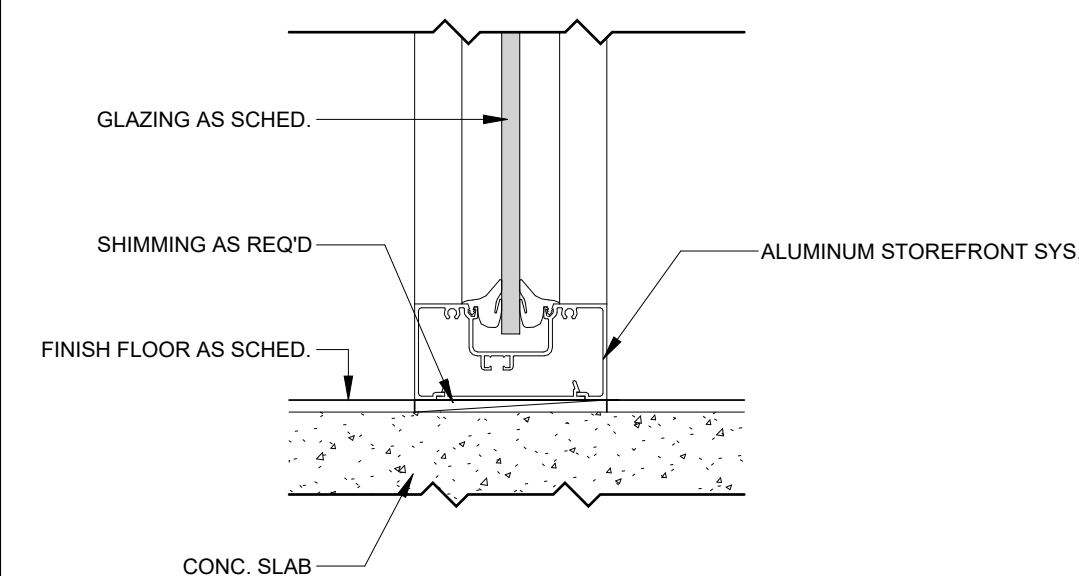
10 Interior Storefront Window Sill 3" = 1' - 0"
