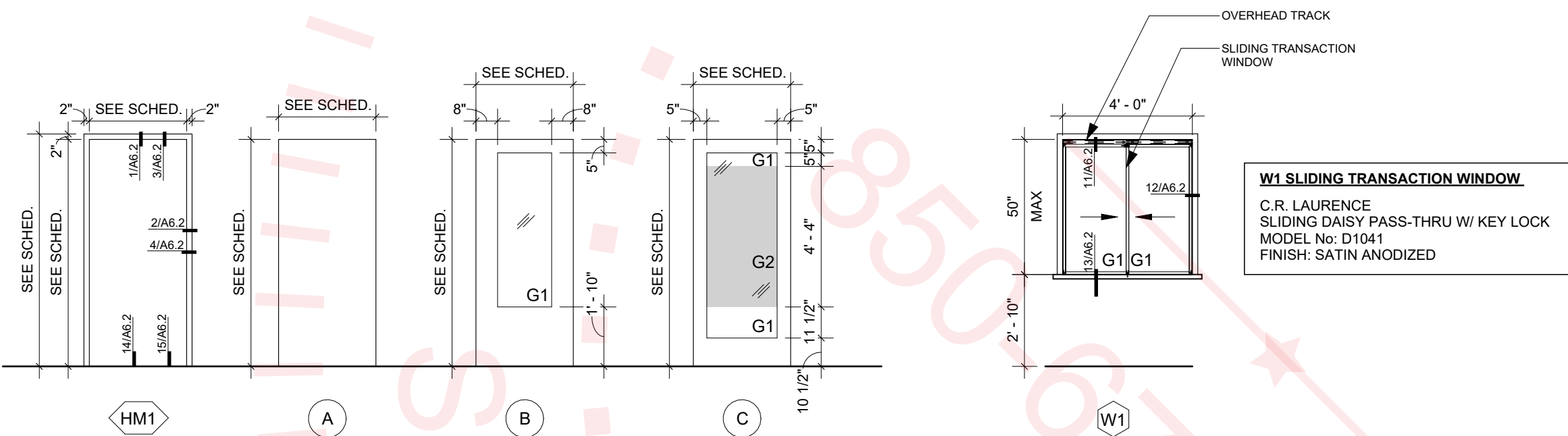
1 Door and Window Elevations 1/4" = 1'-0"
