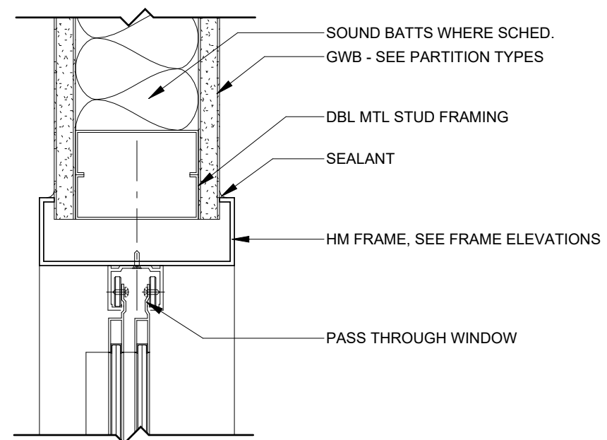
11 Interior HM Pass Through Window Head 3" = 1' - 0"
