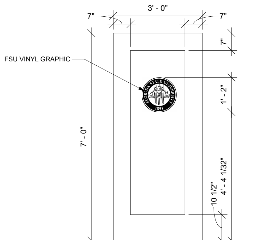
3 Door Graphic Elevation 1/2" = 1'-0"
