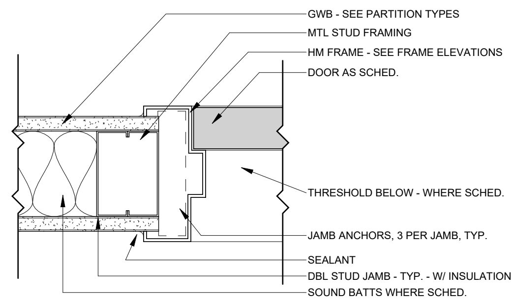
Interior HM Door Jamb 3" = 1' - 0"
