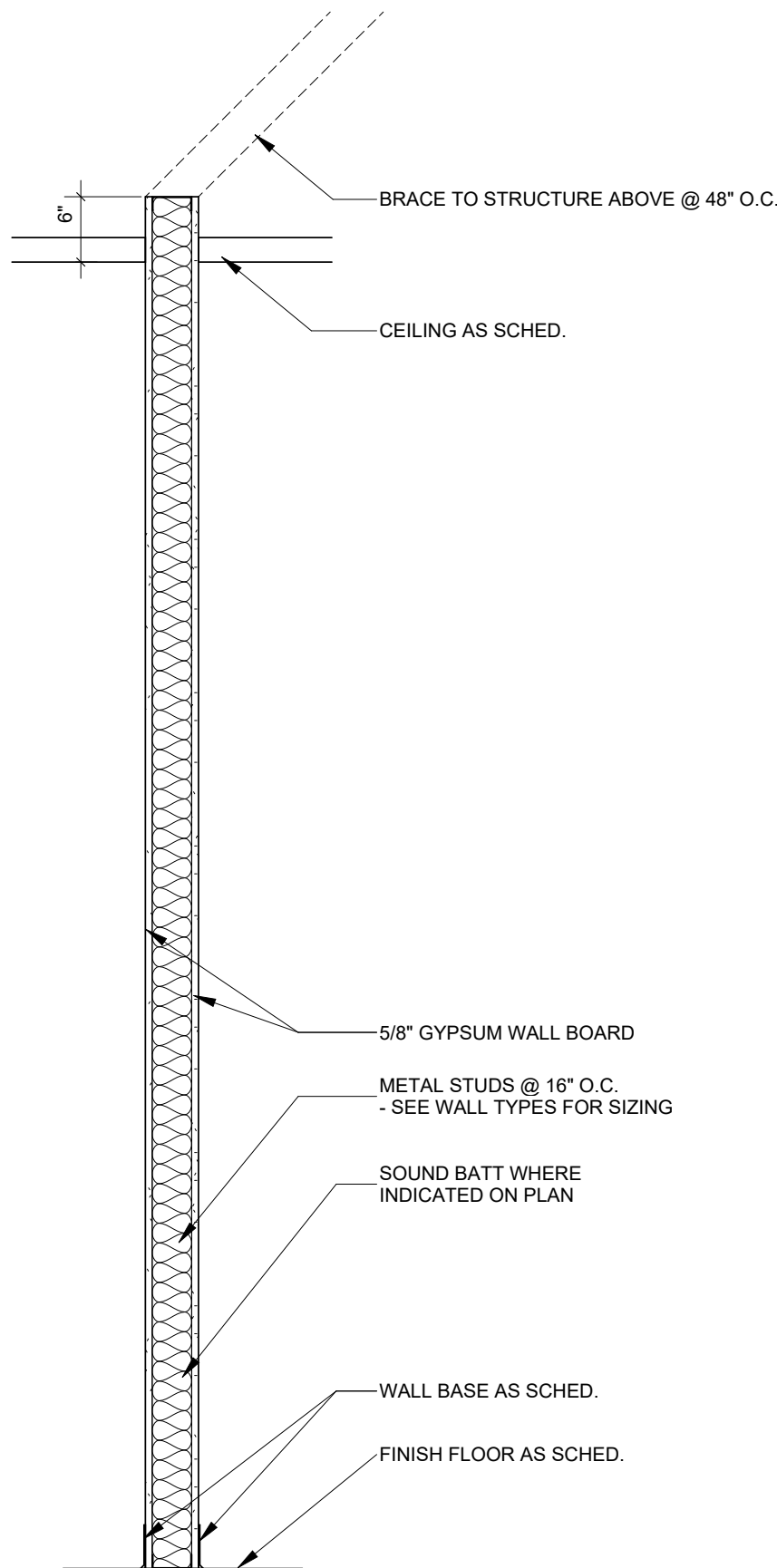
2 Typical Wall Section 3/4" = 1'-0"
