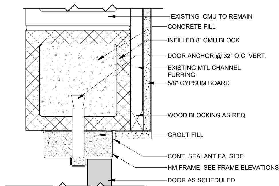
4 Interior HM Door Jamb at CMU Wall 3" = 1' - 0"
