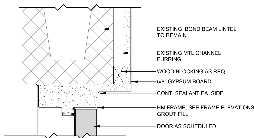
3 Interior HM Door Head at CMU Wall 3" = 1' - 0"
