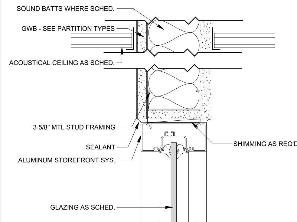
5 Interior Storefront Window Head 3" = 1' - 0"
