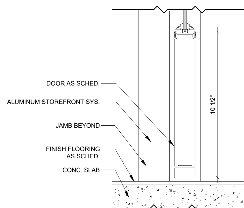
16 Interior Storefront Door Threshold 3" = 1' - 0"
