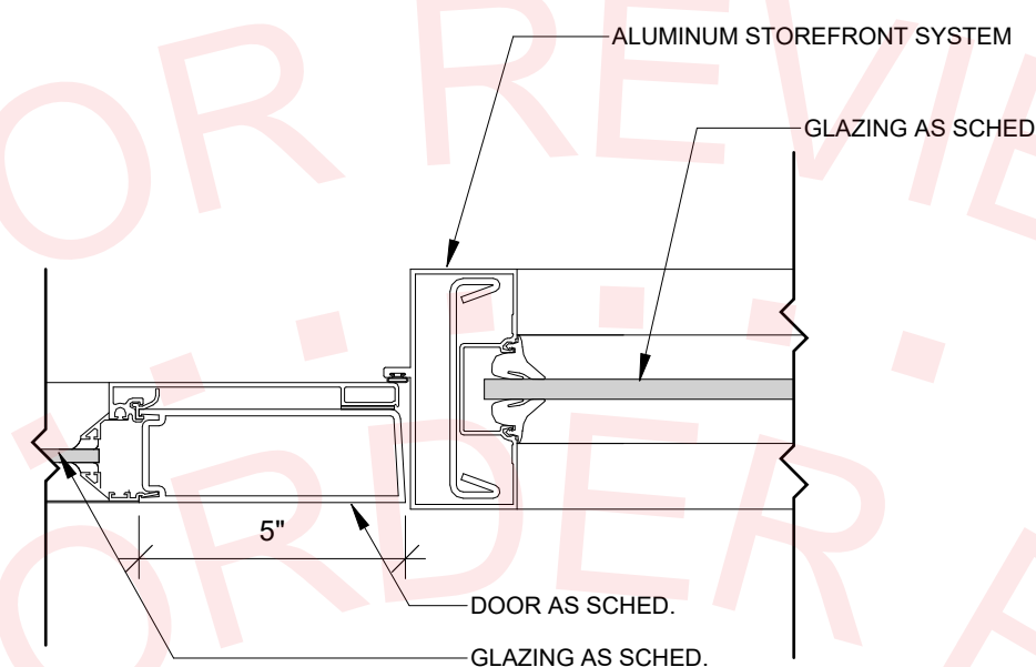
8 Interior Storefront Door / Window Jamb 3" = 1' - 0"
