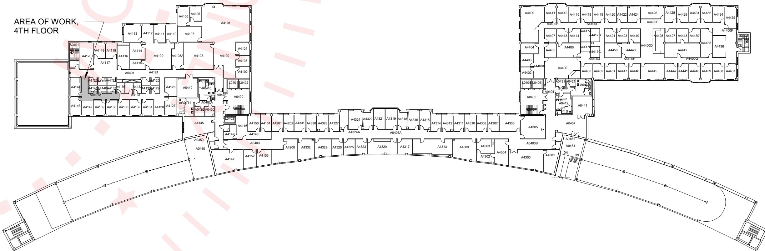
KEY PLAN (4TH FLOOR)
