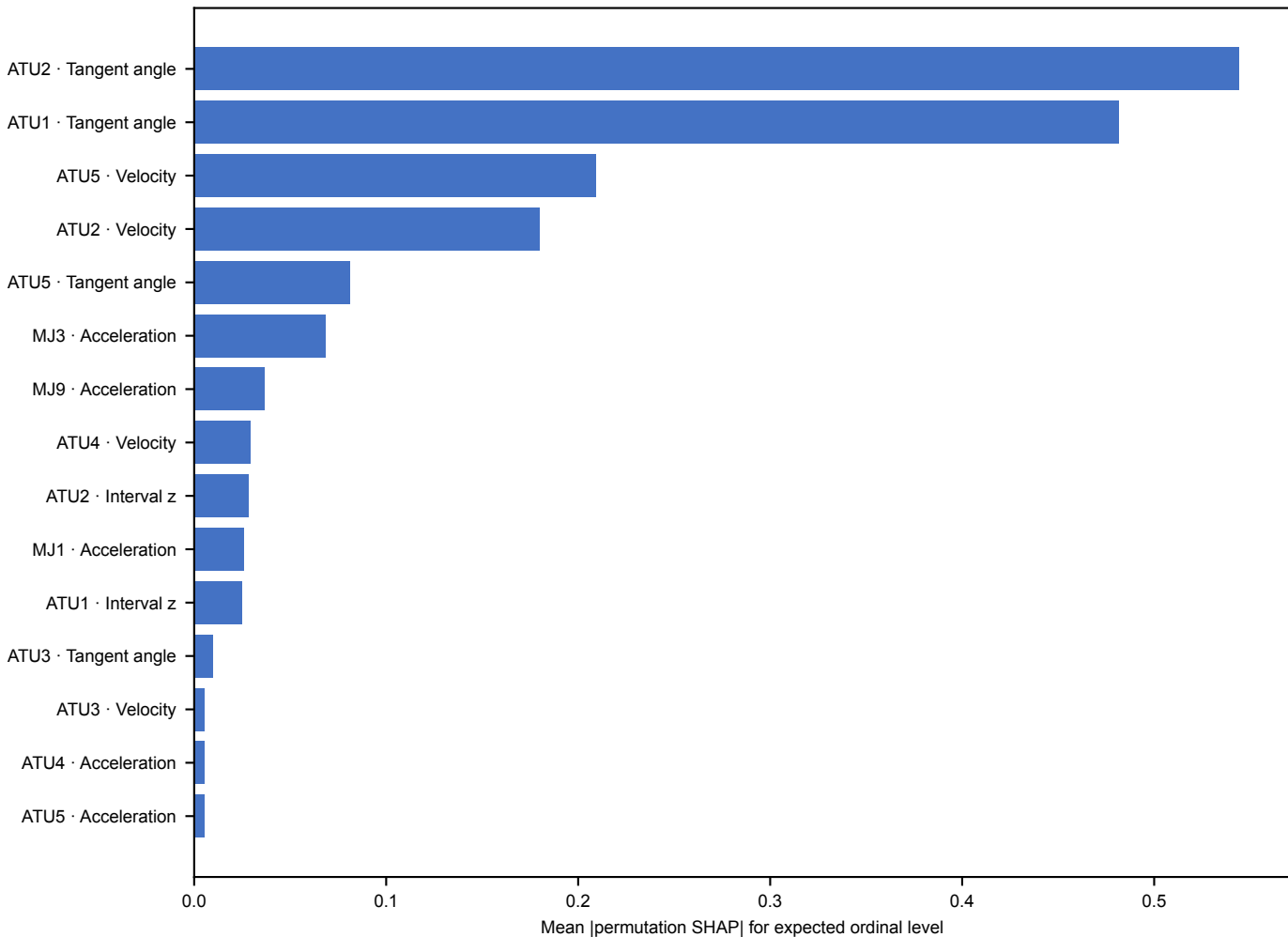
Fold 2 site-model dependence (non-causal)
