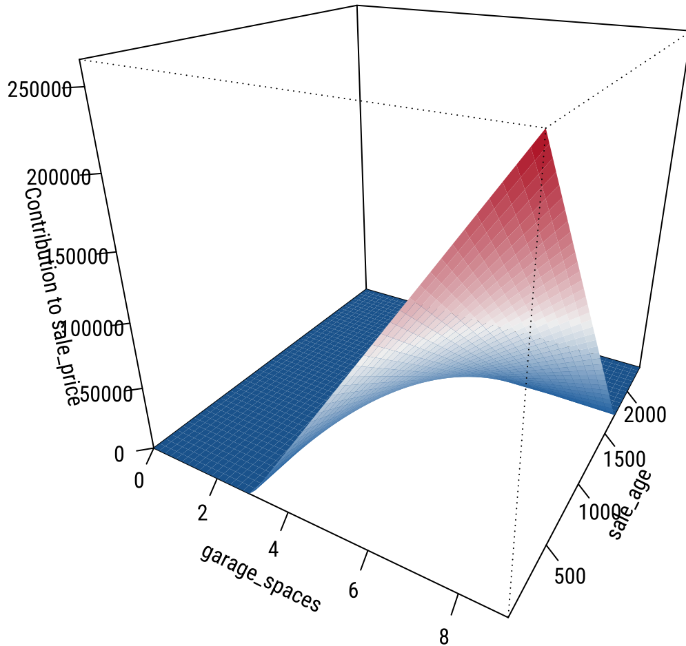
garage_spaces sale_age (1 term)
