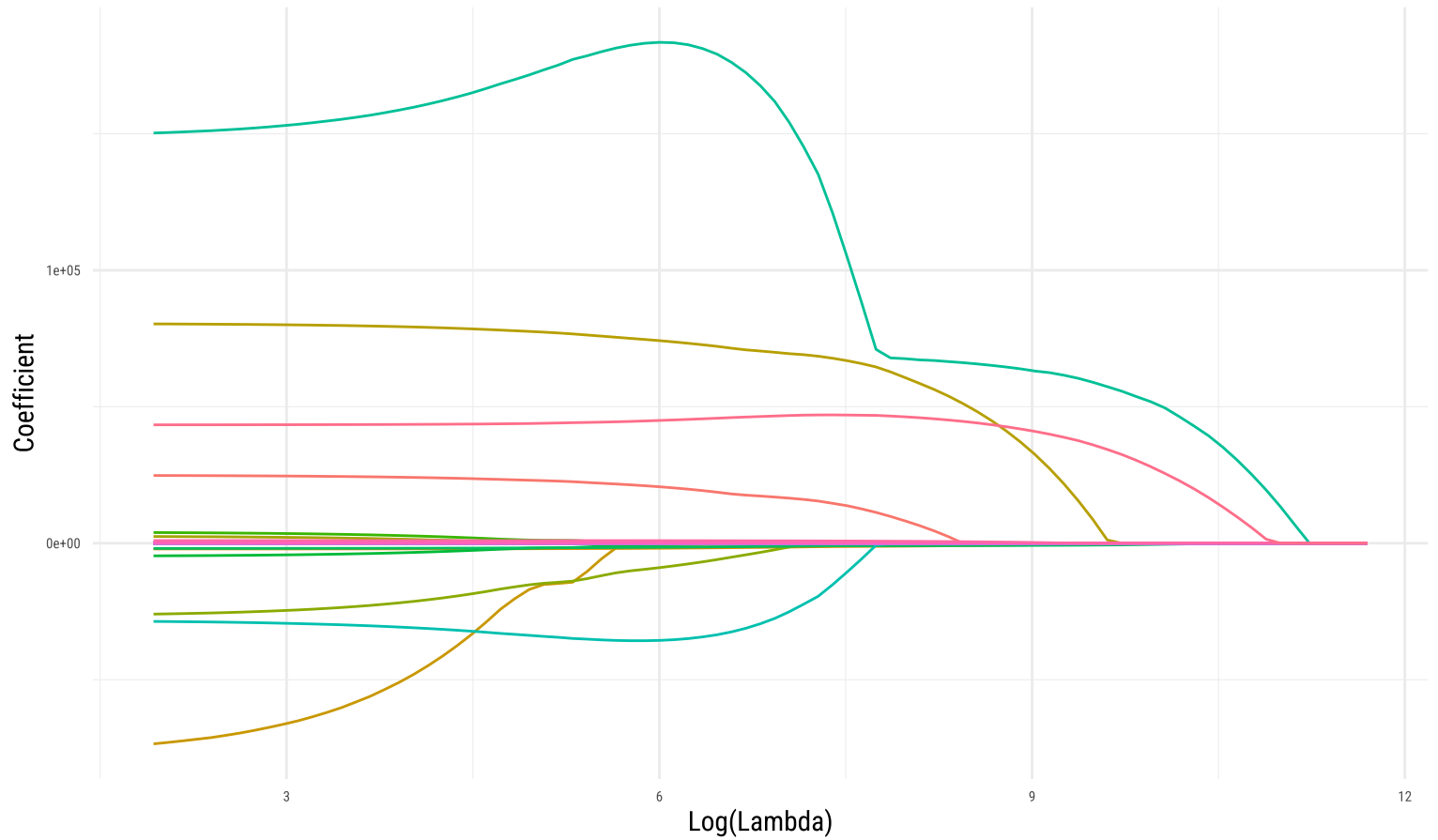
Coefficient Path
