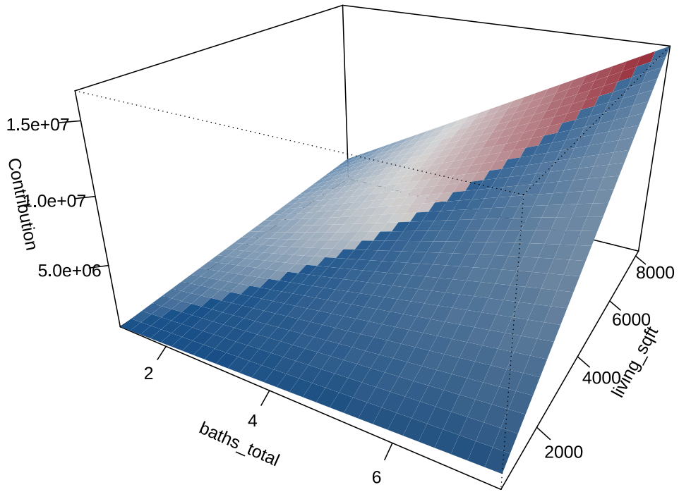
3D Surface: baths_total × living_sqft
