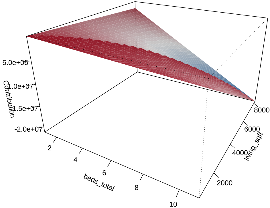
3D Surface: beds_total × living_sqft
