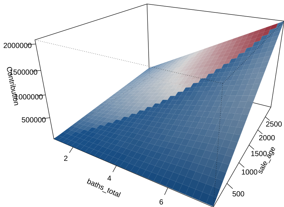
3D Surface: baths_total × sale_age
