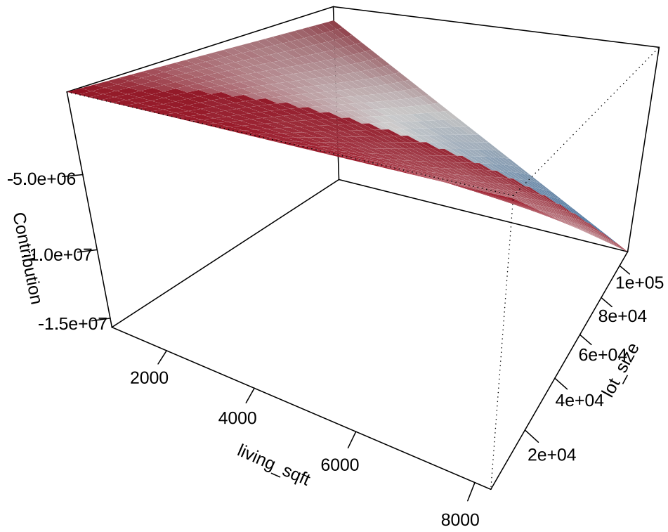
3D Surface: living_sqft × lot_size
