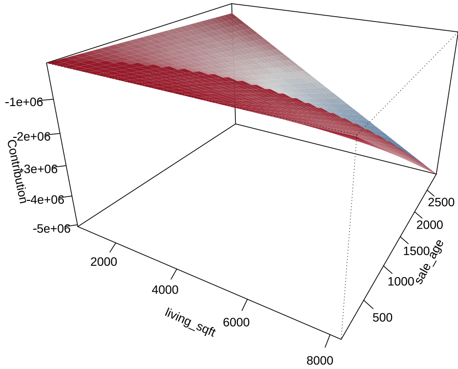
3D Surface: living_sqft × sale_age
