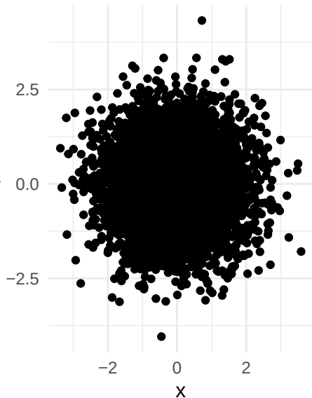
Overplotted
