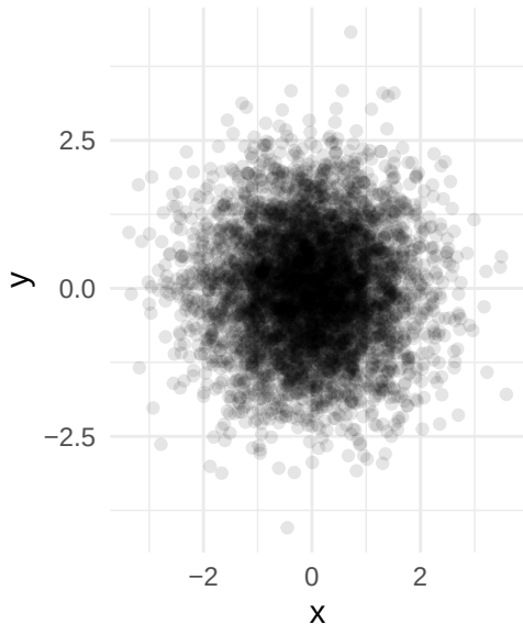
alpha = 0.1
