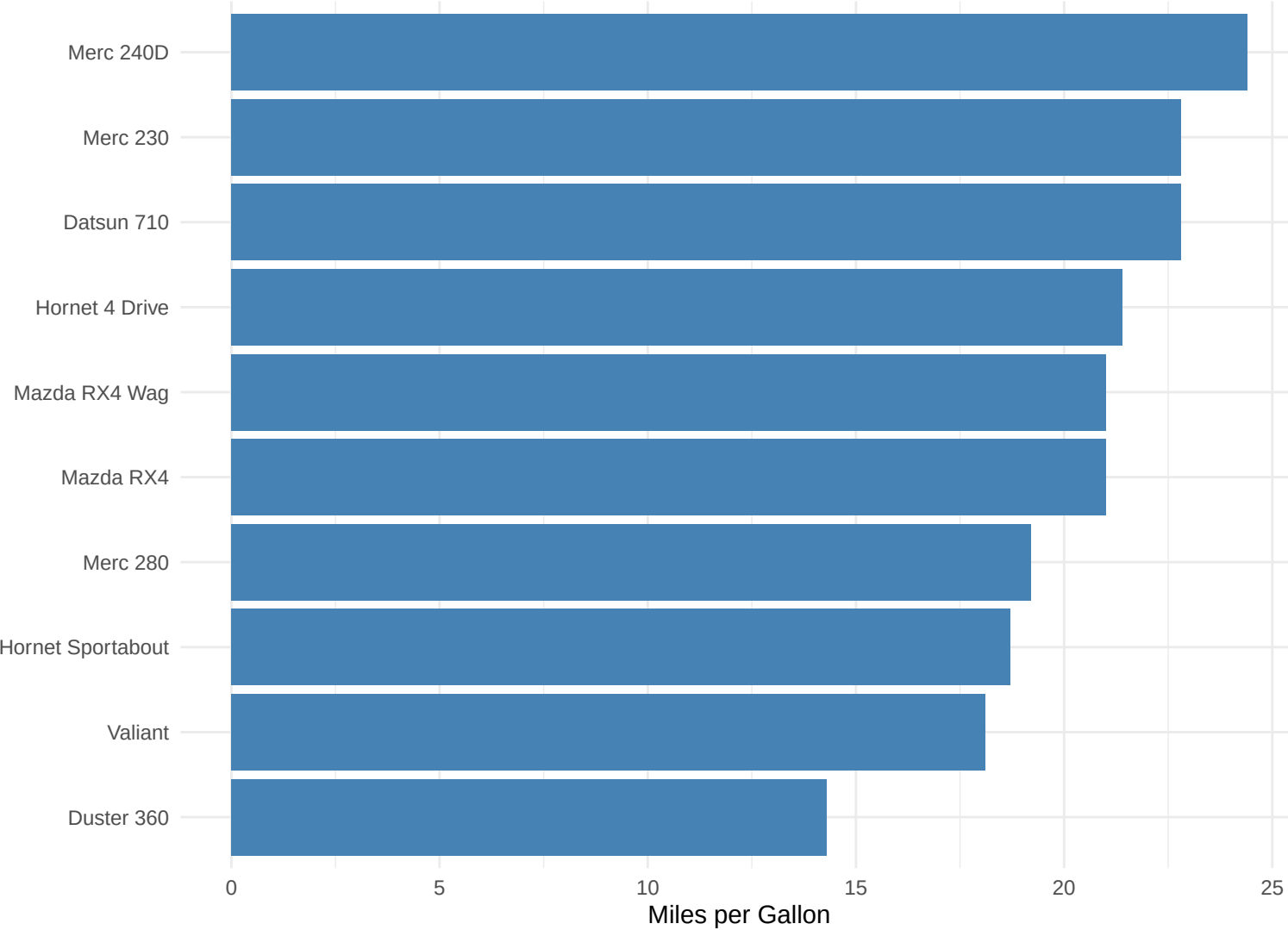
Fuel Efficiency by Car (Ordered)
