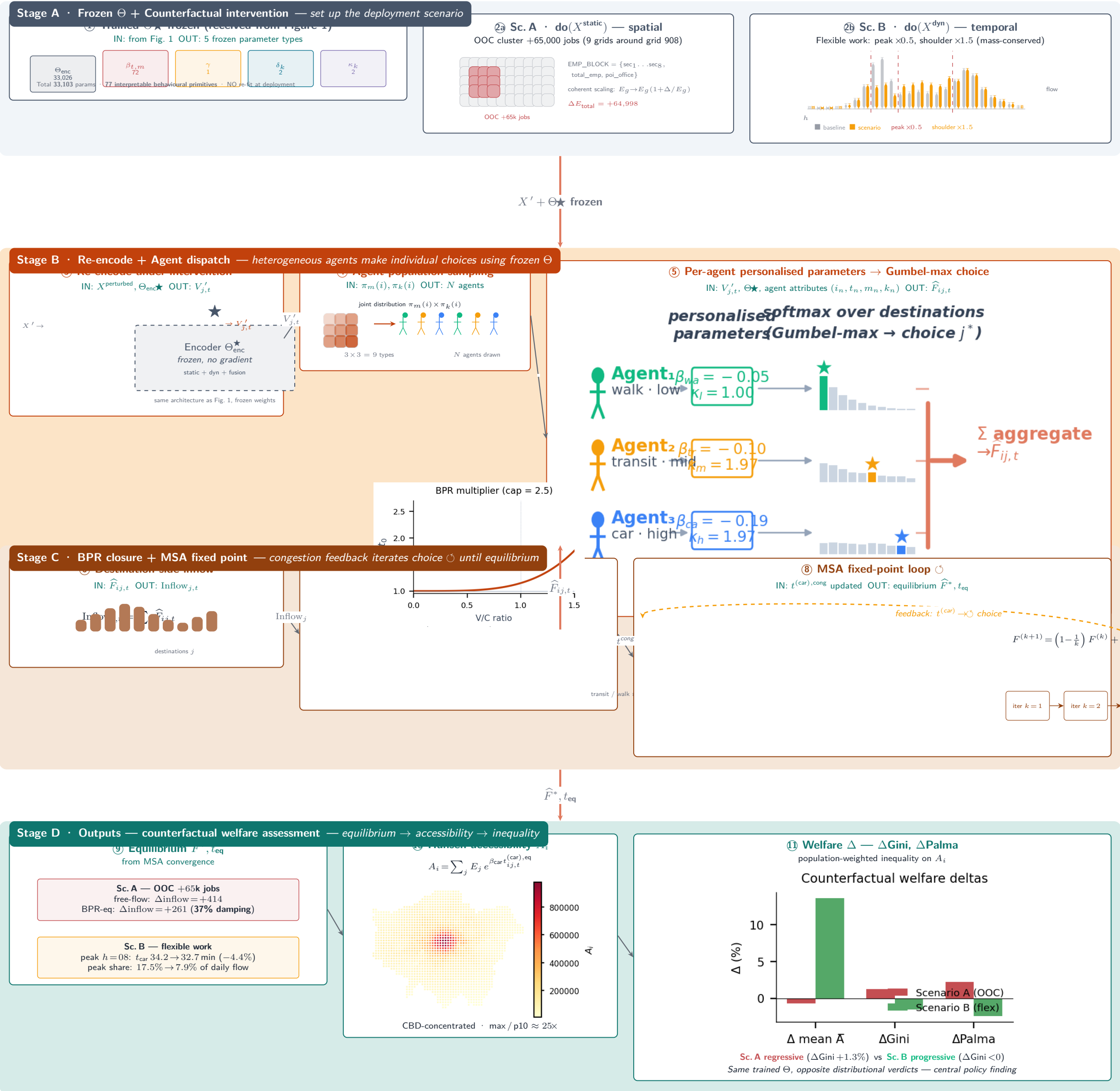
Figure 2 — ABM Forward Simulation Pipeline counterfactual deployment with frozen trained \Theta + destination-side BPR closure
