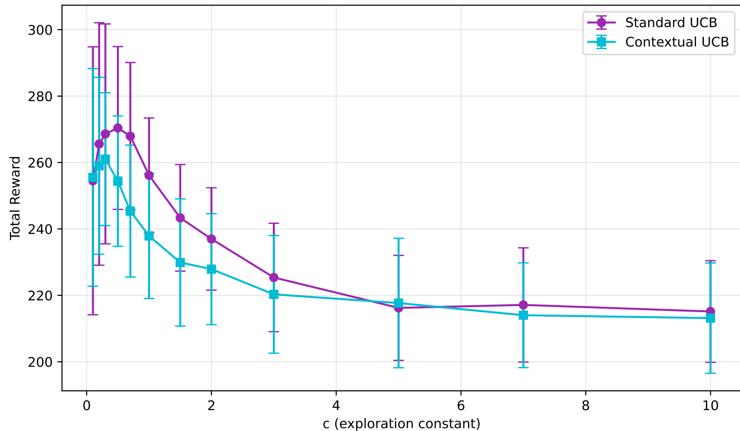
UCB: c vs Total Reward (6-action)
