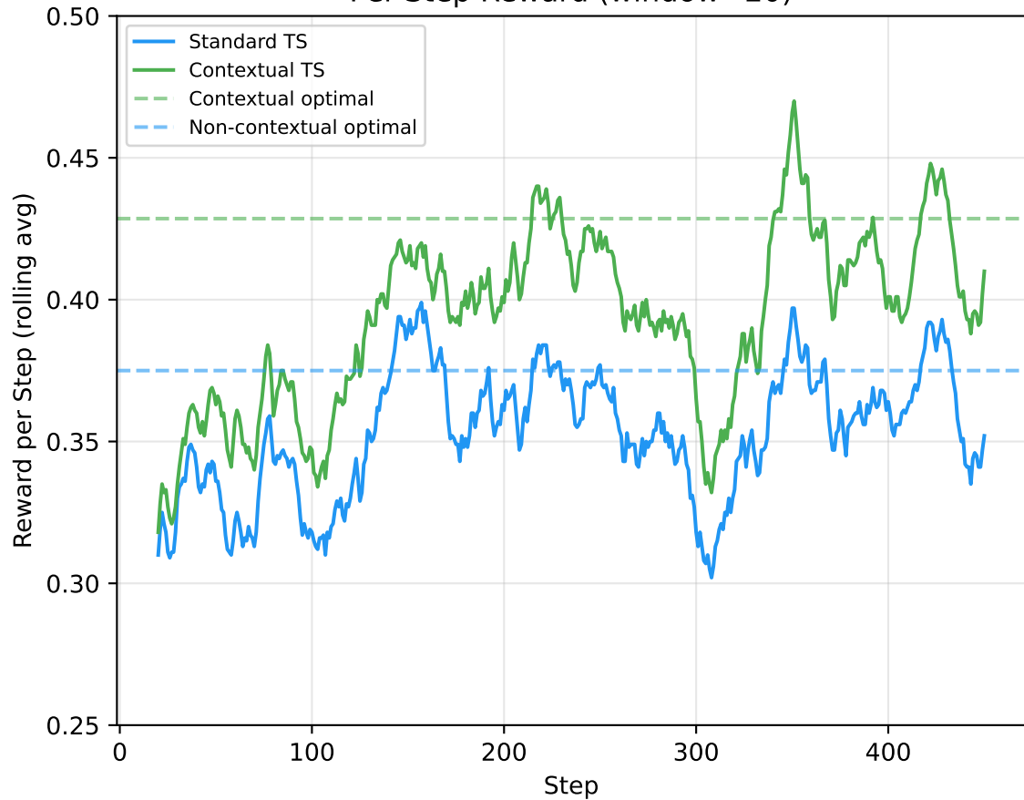
Per-Step Reward (window=20)
