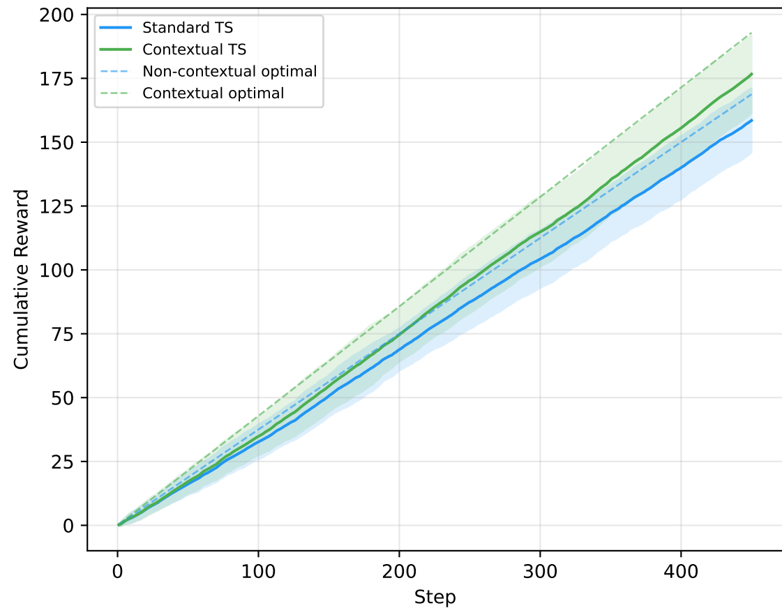
Cumulative Reward
