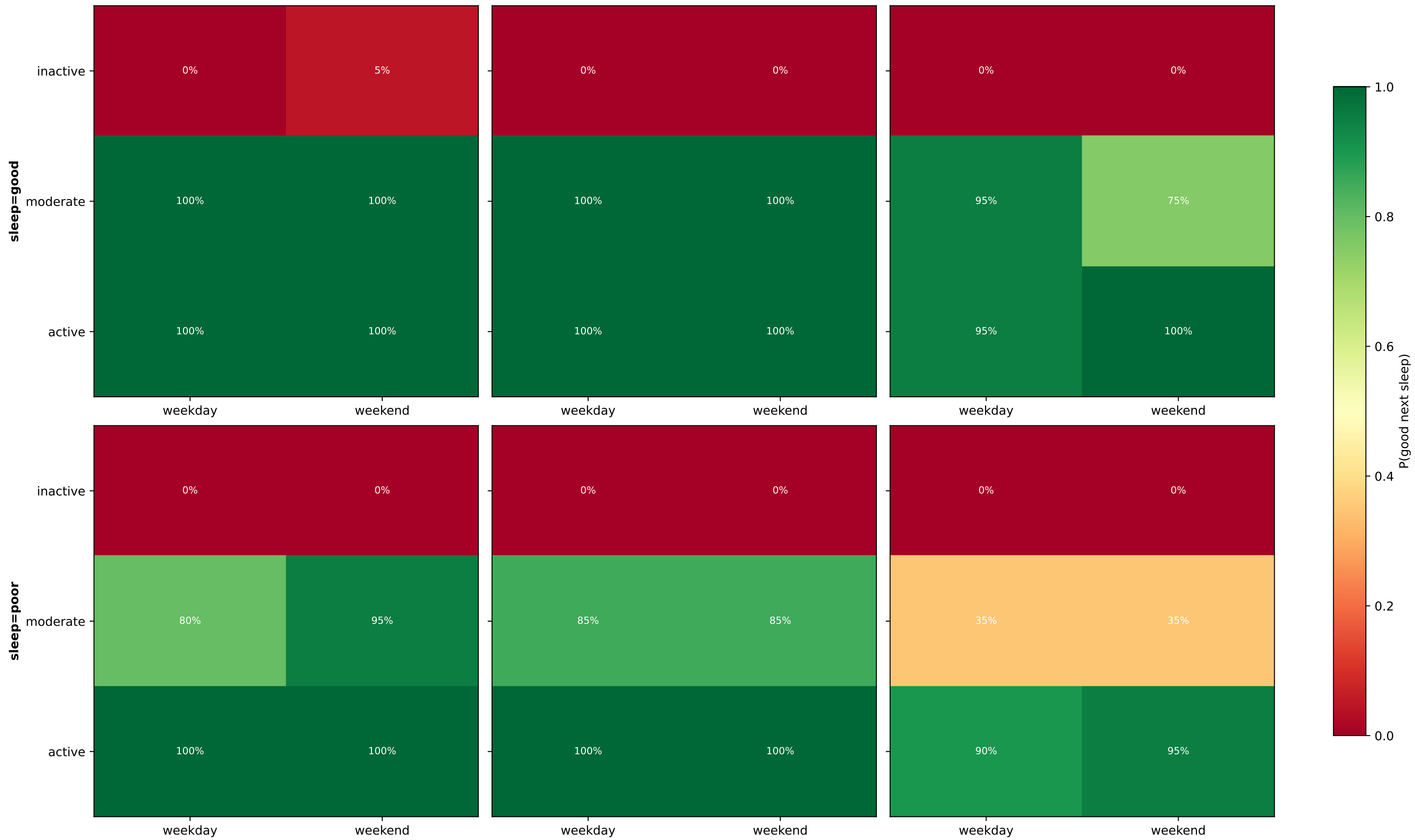
glm5.2 — P(\text{next sleep} = \text{good} \mid \text{step\_bin\_daily}, \text{burden}, \text{day\_type}, \text{sleep}) Rows: current sleep. Columns: burden level (low, medium, high). Realistic: poor sleep or higher burden reduces P(\text{good}) .
