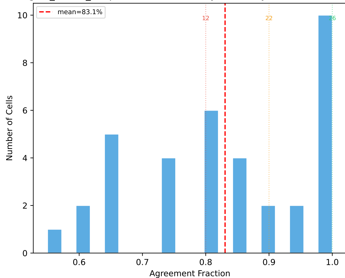
goal_driven_deepseek-v4-flash — Day Boundary Cell Consistency
