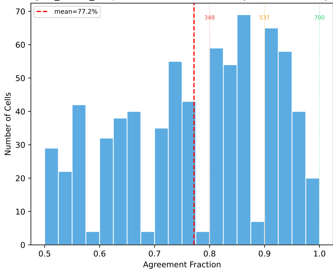
goal_driven_deepseek-v4-flash — Within Day Cell Consistency
