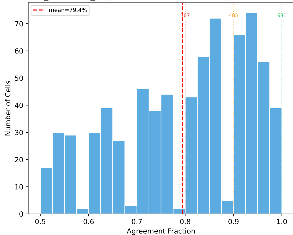
social_responder_deepseek-v4-flash — Within Day Cell Consistency
