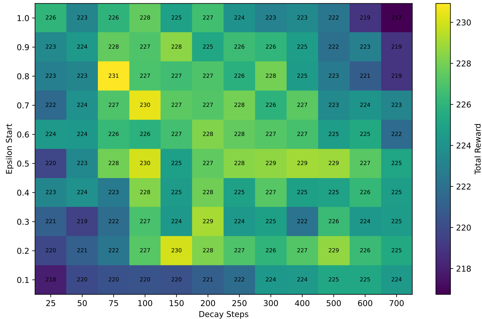
Standard DEC: Total Reward
