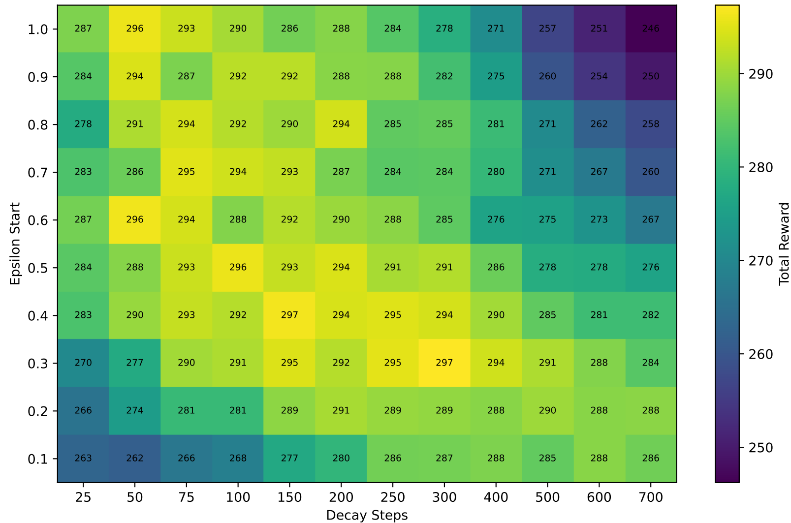
Contextual DEC: Total Reward
