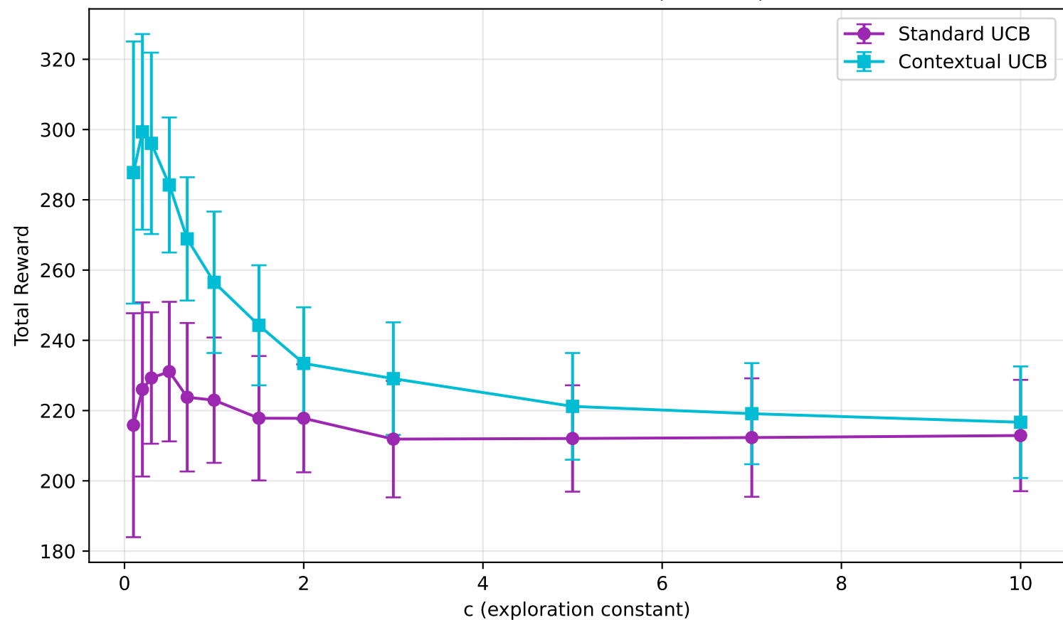
UCB: c vs Total Reward (6-action)
