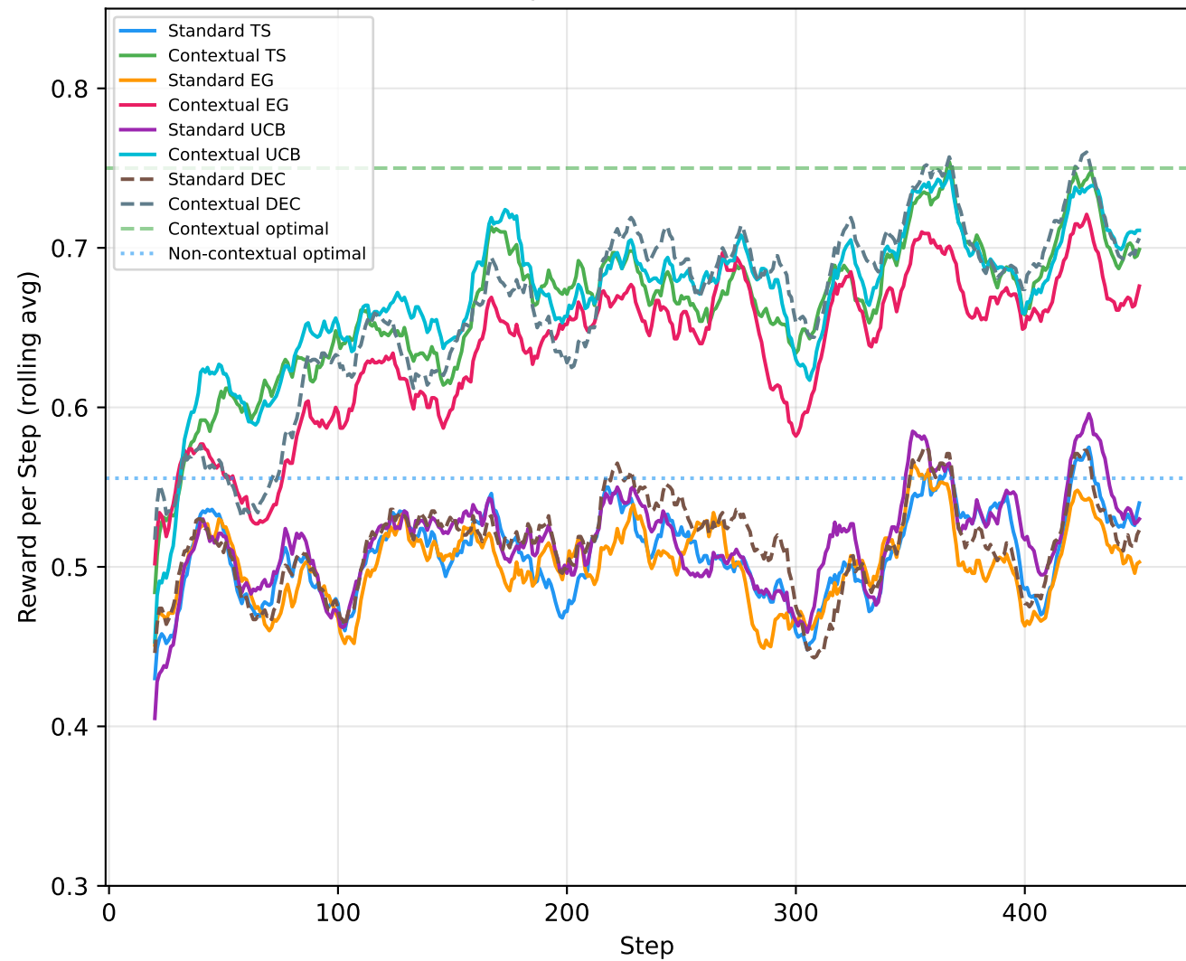
Per-Step Reward (window=20)
