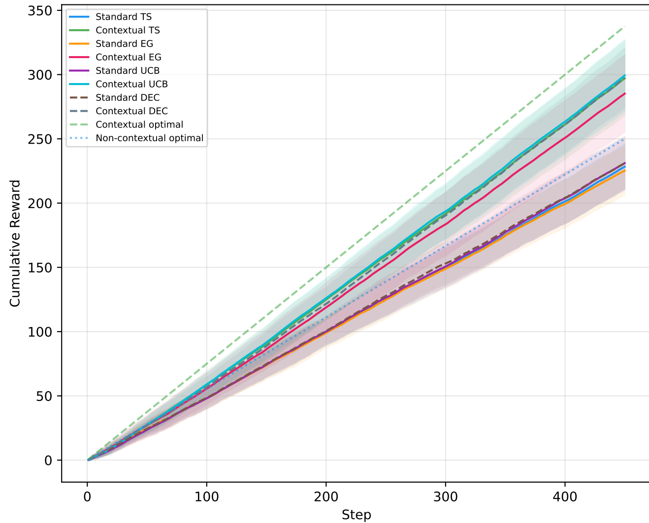
Cumulative Reward (6-action)
