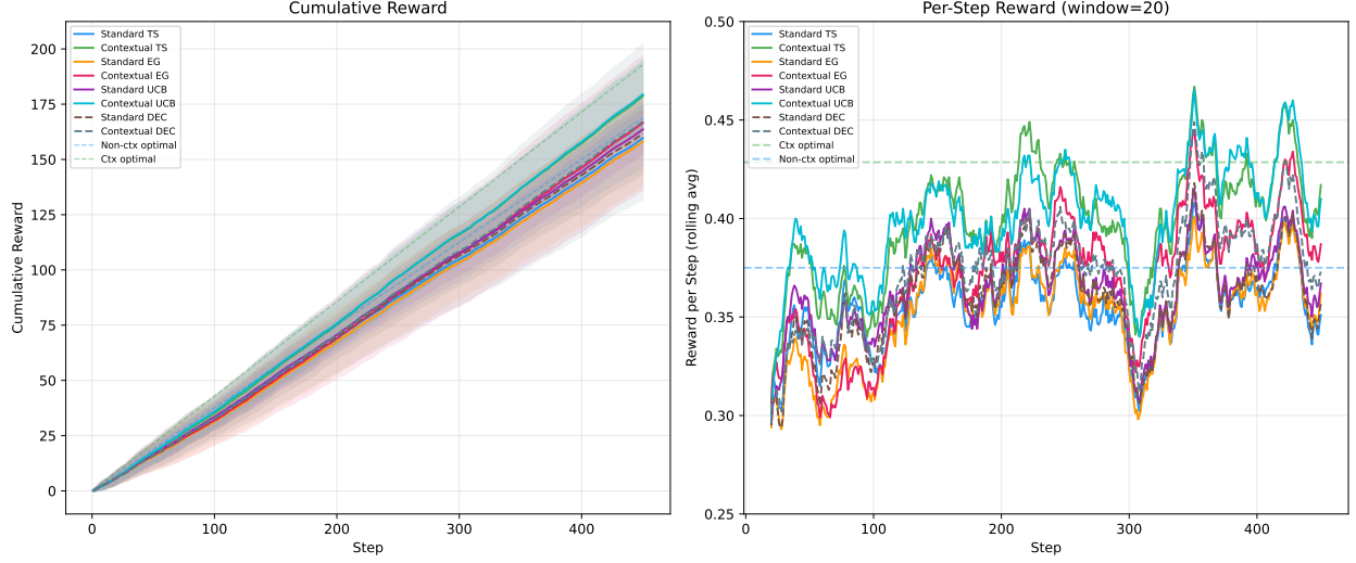
Figure 1: Left: cumulative reward (50 seeds, \pm 1 SD). Right: per-step reward (20-step rolling avg). Contextual agents converge toward 3/7 \approx 0.429 ; standard agents plateau at lower rates. The decaying-epsilon variants (DEC) show higher variance during early exploration but narrow the gap with their fixed-epsilon counterparts.
