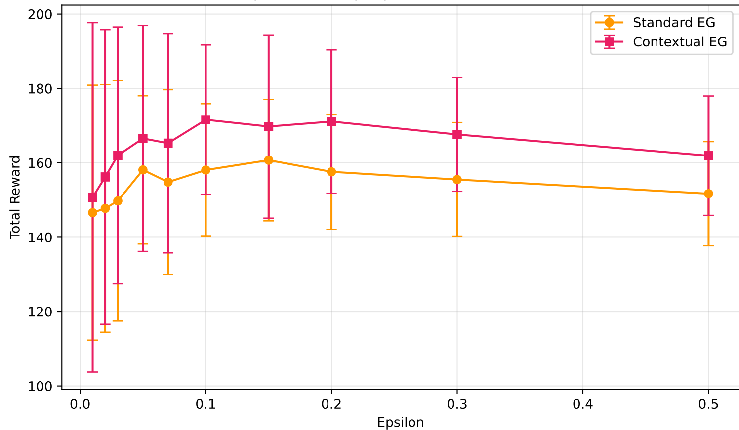
Epsilon-Greedy: Epsilon vs Total Reward
