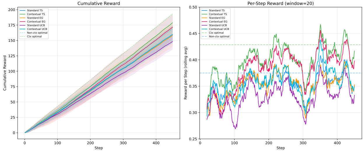
Figure 1: Left: cumulative reward (50 seeds, \pm 1 SD). Right: per-step reward (20-step rolling avg). Contextual agents converge toward 3/7 \approx 0.429 ; standard agents plateau at lower rates.
