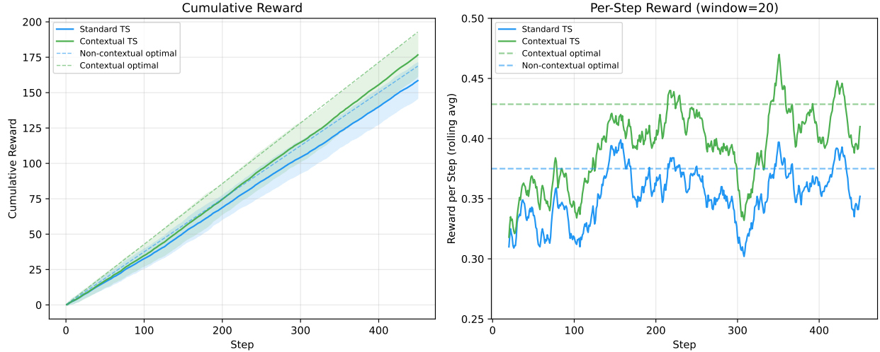
Figure 1: Left: cumulative reward over 450 steps (50 seeds, shaded \pm 1 SD). Right: per-step reward (20-step rolling average). Contextual TS converges toward the contextual upper bound ( 3/7 \approx 0.429 ) by the final steps, while standard TS plateaus near the non-contextual optimal (0.375).
