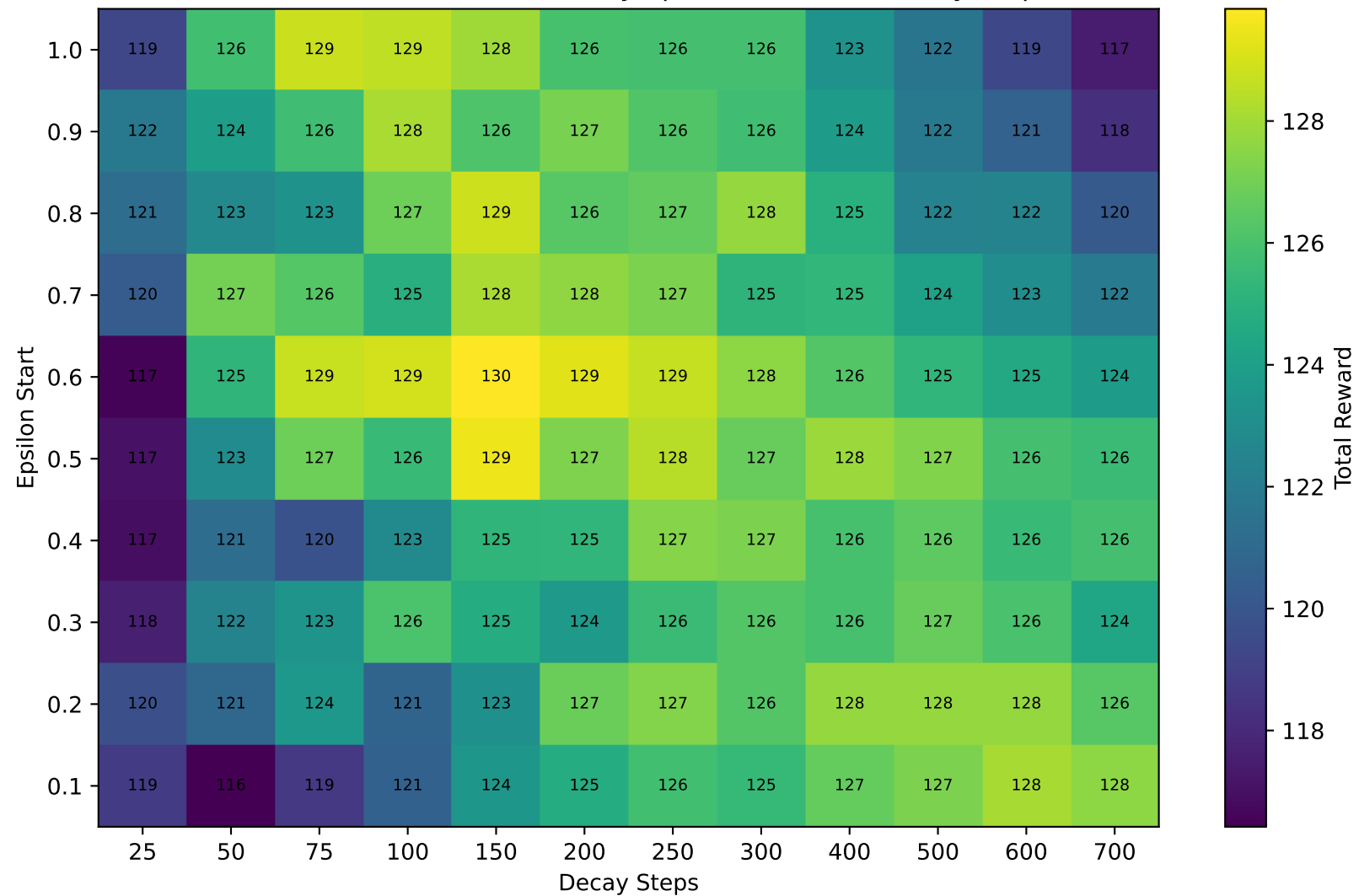
Standard D-EG: Total Reward by Epsilon Start and Decay Steps
